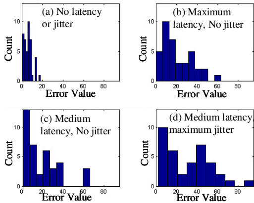
Figure 7: The distribution of errors increases with increasing latency and jitter.
