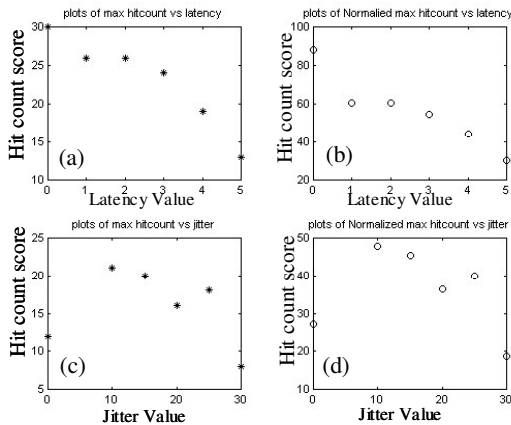
Figure 3(a)-(d): As latency is increased, the participant’s success at scoring a hit reduces. Introducing jitter also results in a significant reduction.
