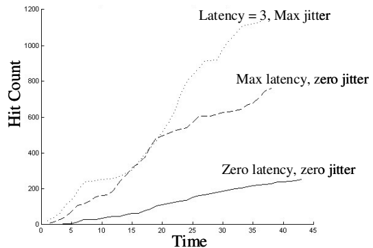
Figure 5: As time progresses the cumulative absolute error increases but does so more rapidly in the presence of jitter than that of latency.
