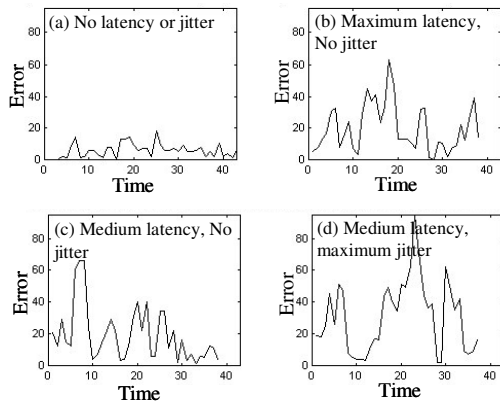
Figure 6(a)-(d): Plots of instantaneous error for different latency/jitter combinations
