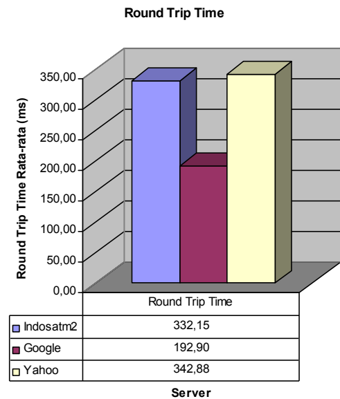
Gambar 10. Grafik Round Trip Time Rata-rata
