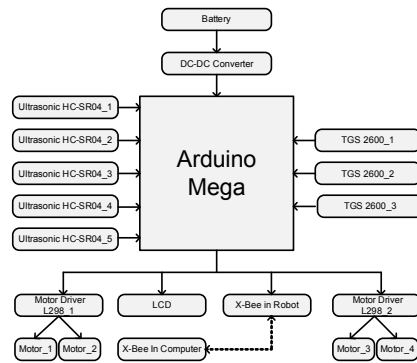
Fig. 3. Block Diagram of Odor Localization Robot
