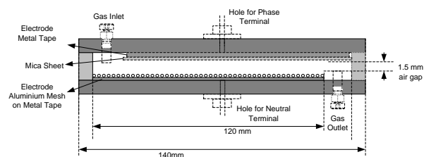
Figure 1. Ozone chamber
