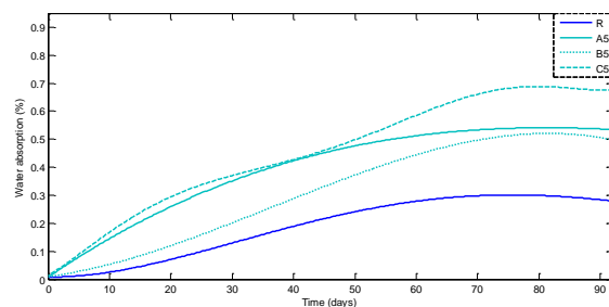
Fig. 11: Percentage of water absorption for SiO 2 , TiO 2 and MMT at 5% nanofiller
