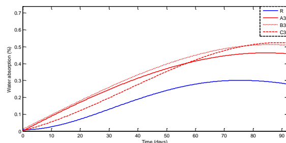
Fig. 10: Percentage of water absorption for SiO 2 , TiO 2 and MMT at 3% nanofiller
