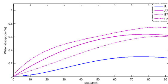
Fig. 12: Percentage of water absorption for SiO 2 , TiO 2 and MMT at 7% nanofiller
