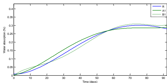
Fig. 9: Percentage of water absorption for SiO 2 and TiO 2 at 1% nanofiller
