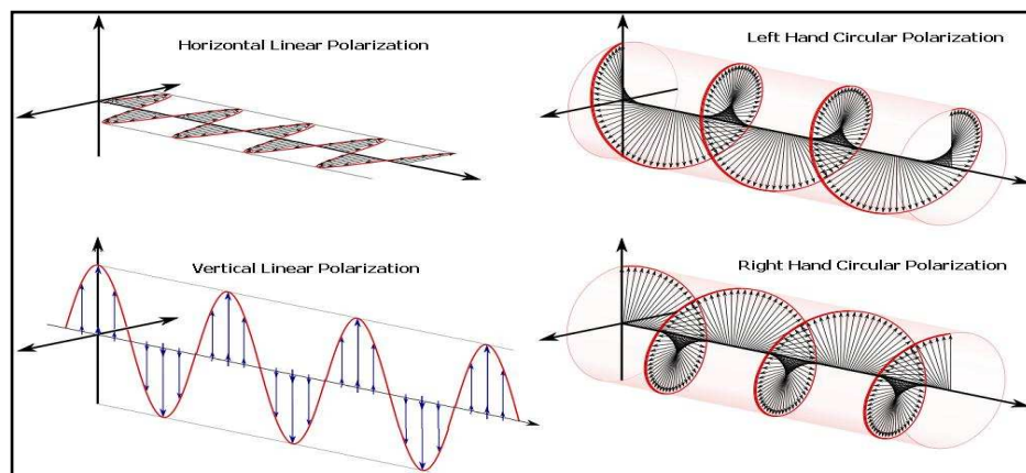
Fig. 3: Schematic diagram of linear horizontal, linear vertical, right circular and left circularly polarized signals [Source: arnoldsat.com]
