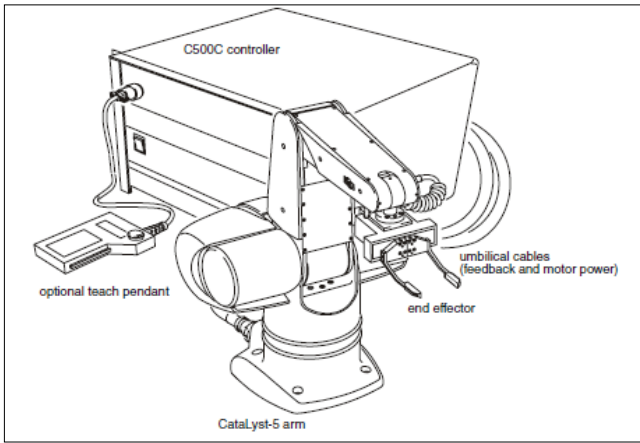
Fig. 1 Basics component of CRS
