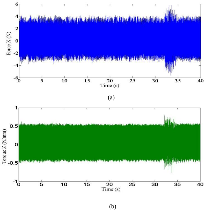
Fig. 8 (a) Force in x-direction (b) Torque in z-direction
