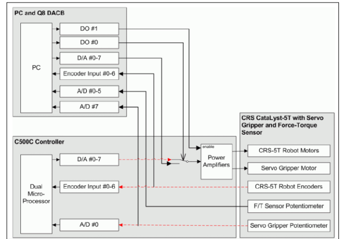
Fig. 2 Closed and open architecture system
