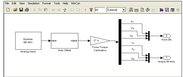
Fig. 4 Force-Torque Sensor subsystem
