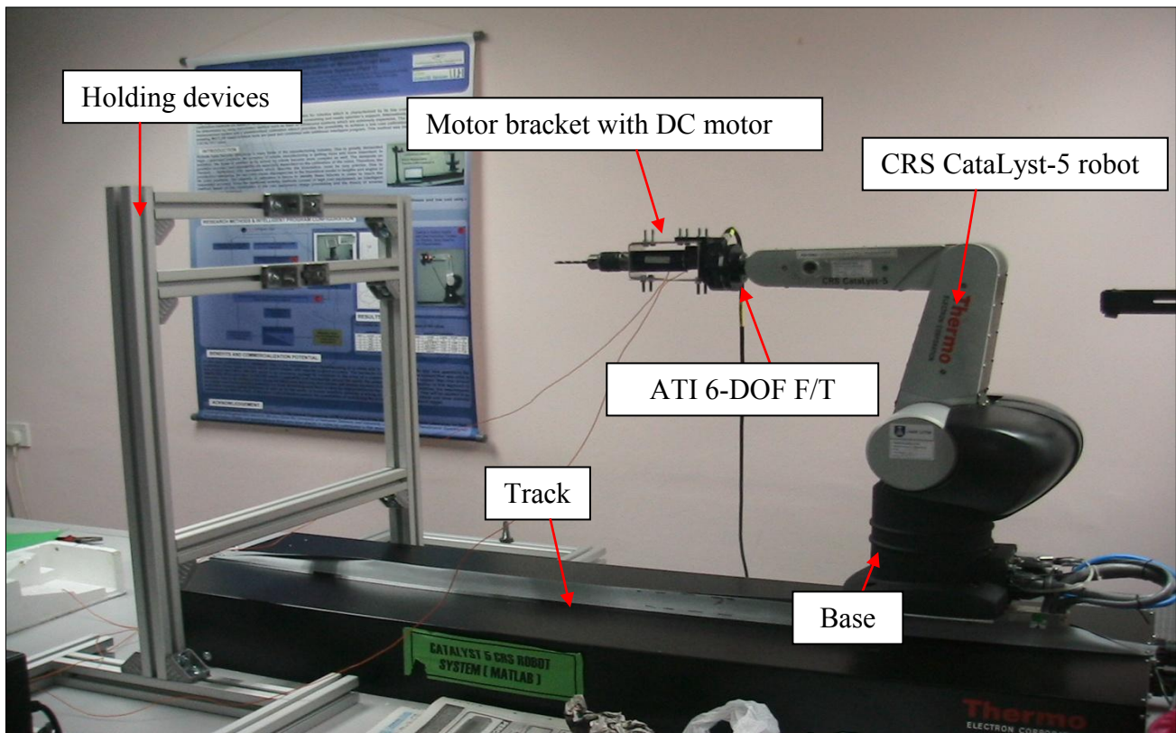
Fig. 5 Real layout drilling operation
