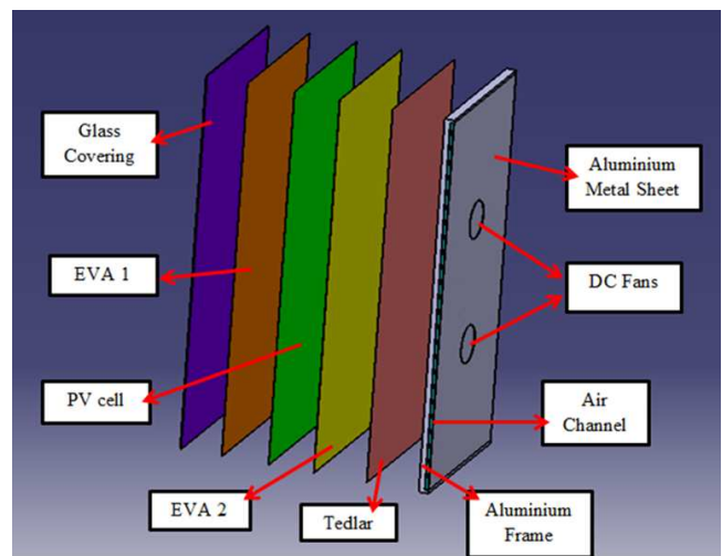
Fig. 1 Sketch of the PV panel geometry model
