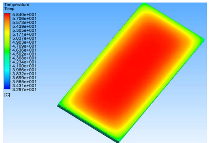
Fig. 4 Temperature distribution of PV panel without cooling system
