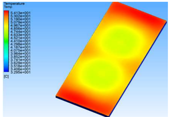
Fig. 5 Temperature distribution of PV panel with 2 m/s of DC fan flow rate
