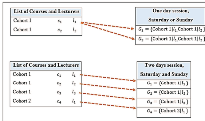
Fig. 3 Group assignment based on teaching slot types.
