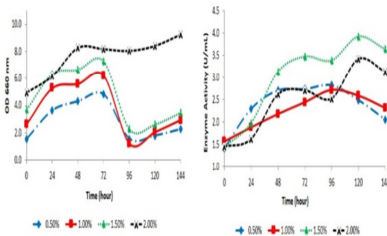
Fig 2. The growth curve (a) and the enzyme activity (b) of Bacillus safensis P20 at various substrate concentration
