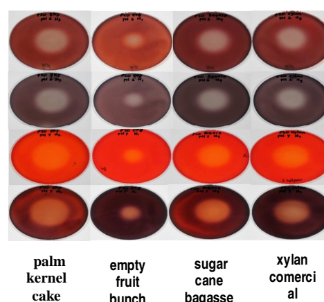
Fig 1. Data of clear zone from three biomass (palm cernel cake, empty fruit bunch and sugar cane bagasse VS xylan commercial) by marine bacterium Bacillus safencis P20
