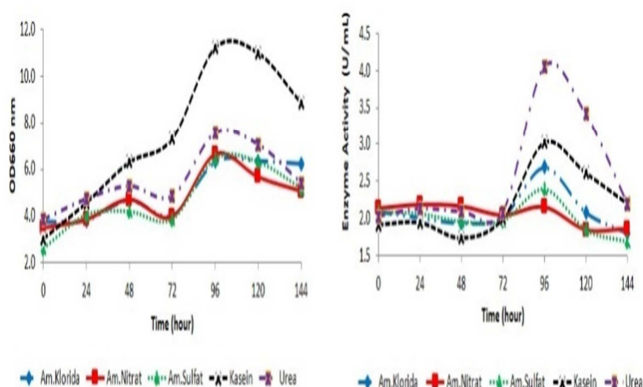
Fig 6. The effect of nitrogen source on growth curve (a) and xylanase activity (b) of Bacillus safensis by using sugarcane bagasse as substrate
