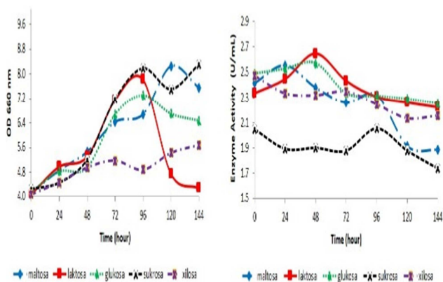
Fig 5. The effect of carbone source on growth curve (a) and the enzyme activity (b) of Bacillus safensis by using sugarcane bagasse as substrate
