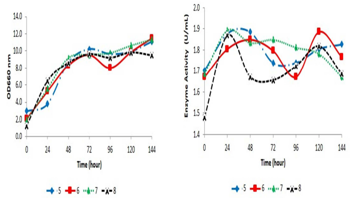
Fig 3 The Growth cell (a) and the enzyme activity (b) of Bacillus safensis P20 on 1.5% sugarcane bagasse at various pH medium
