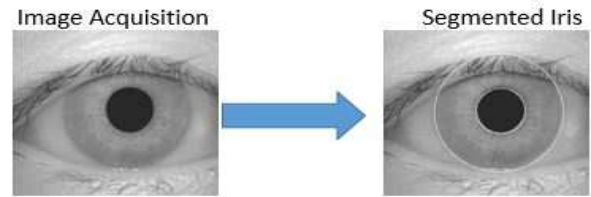
Fig.4. Segmented Iris
