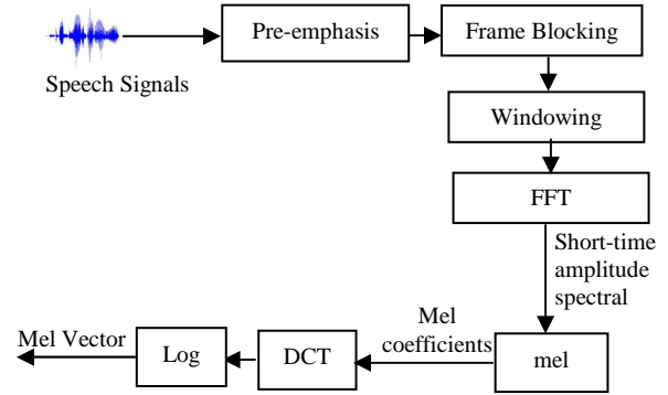
Fig 4. Block diagram of speech analysis procedure
