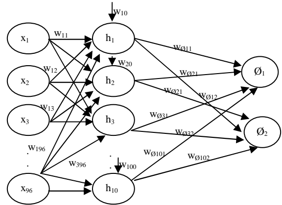
Fig 6. The architecture of BPNNs
