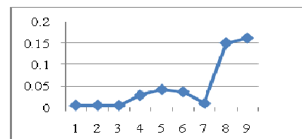
Fig 7. MSE using the various numbers of hidden nodes.
