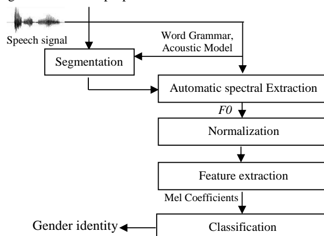
Fig 2. Block diagram of the proposed model
