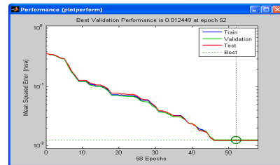
Fig 9. The performance of the system in the testing phase
