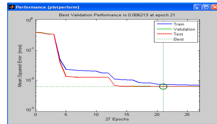
Fig 8. The performance of the system in the training phase
