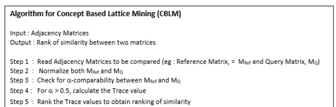
Fig. 7 CBLM Algorithm
