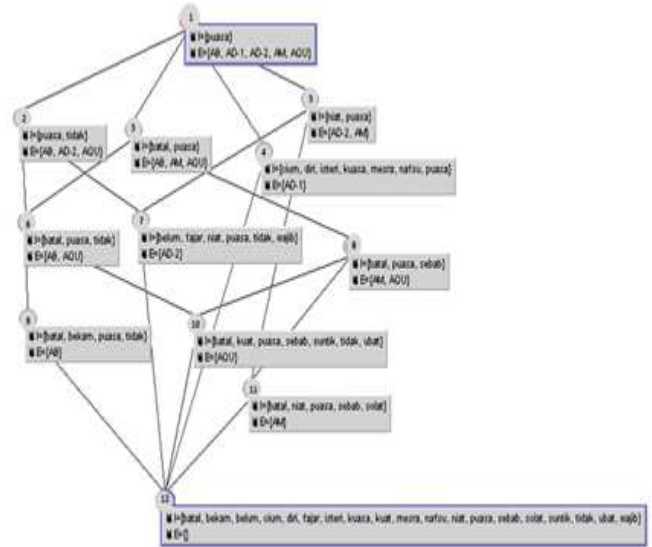
Fig. 9 Output lattice based on Fig. 8
