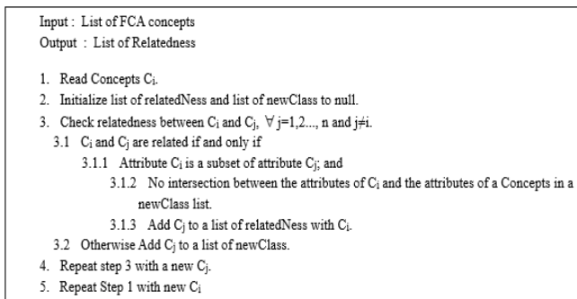
Fig. 4 Relatedness algorithm
