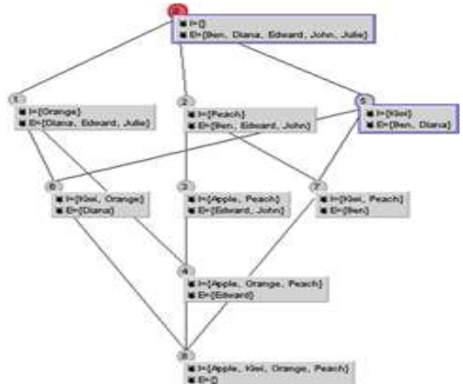
Fig. 3 Galicia lattice output based on input in Fig. 1
