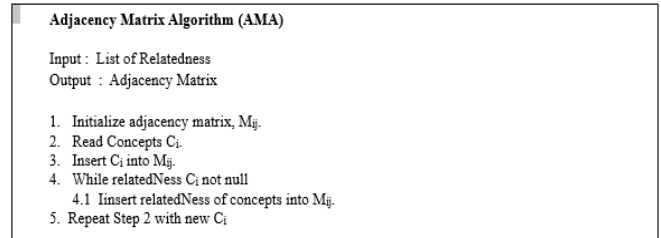
Fig. 5 Adjacency matrix algorithm
