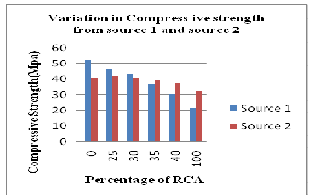
Fig. 3 Compressive strength results from source 1 and source 2
