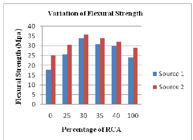
Fig. 4 Comparison of 28 days Flexural strength
