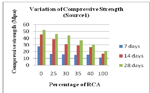
Fig. 1 Compressive Strength Test Results from Source 1
