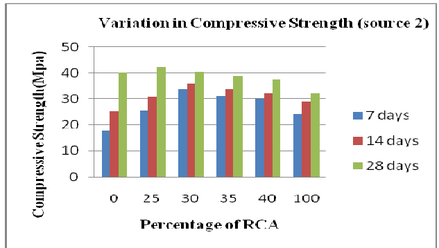
Fig. 2 Compressive Strength test results from source 2
