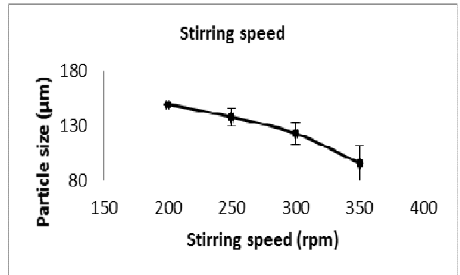
Fig. 6 Effect of stirring speed on microcarrier particle size
