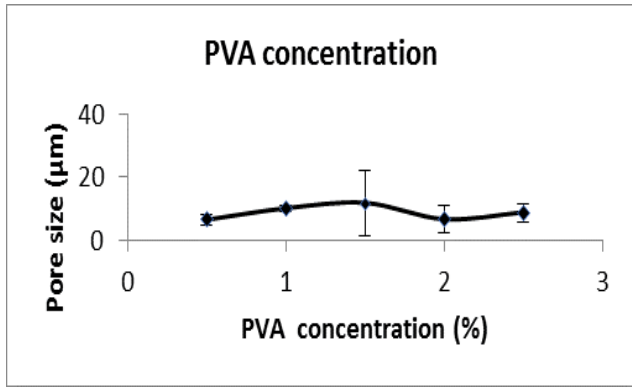
Fig. 2 Effect of PVA concentration on the pore size
