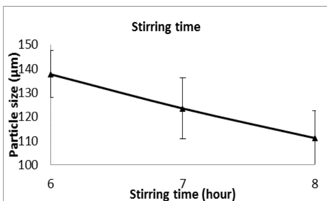
Fig. 9 Effect of stirring time on micro-carrier particle size
