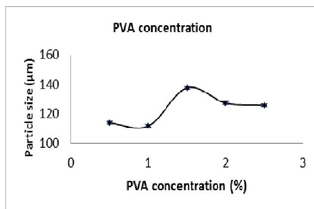
Fig. 1 Effect of PVA concentration on the particle size
