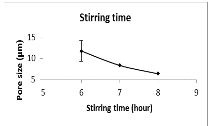
Fig. 10 Effect of stirring time on micro-carrier pore size
