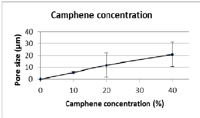
Fig. 3 Effect of camphene percentage on pore size
