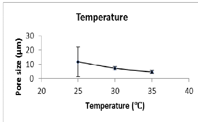
Fig. 8 Effect of temperature on microcarrier pore size
