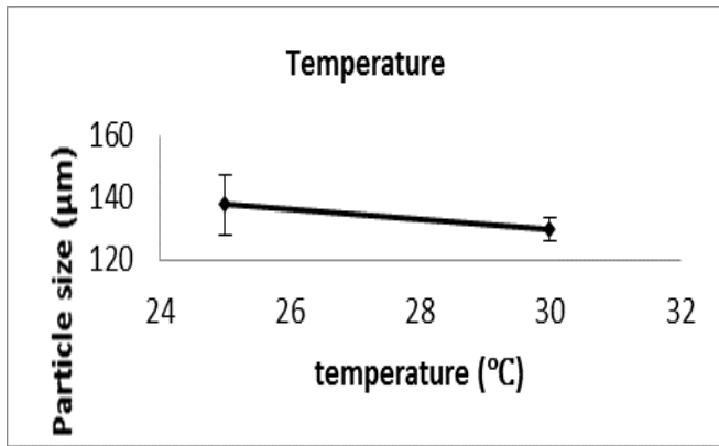
Fig. 7 Effect of temperature on microcarrier particle size
