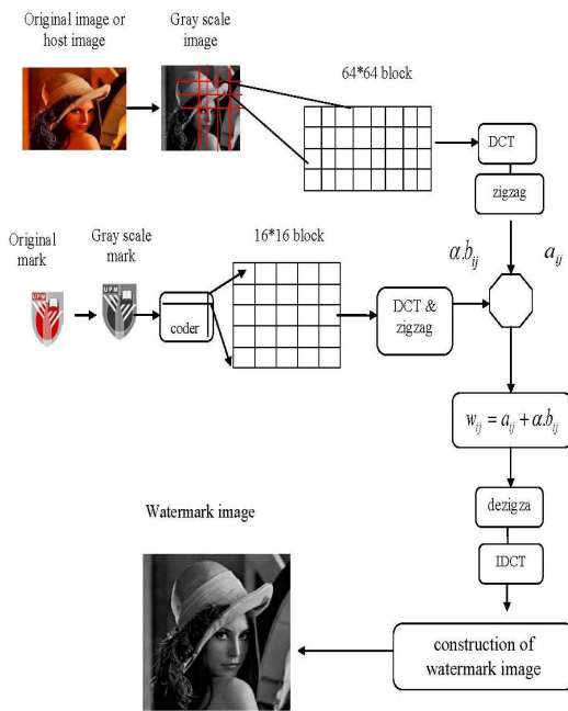
Figure3: watermark embedding system
