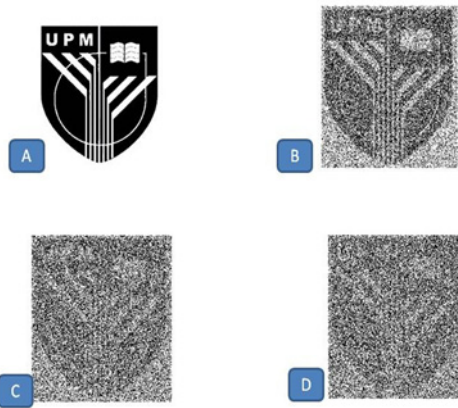
Figure 10 The extracted watermarks from the Gaussian noise contaminated watermarking images
