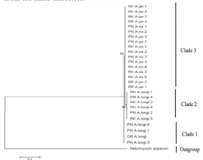
Fig. 4. Maximum Likelihood (ML) phylogenetic tree of Anaphalis at Bromo Tengger Semeru National Park based on ITS sequences. The value on the branch represent bootstrap value based on 1000 replicate.
