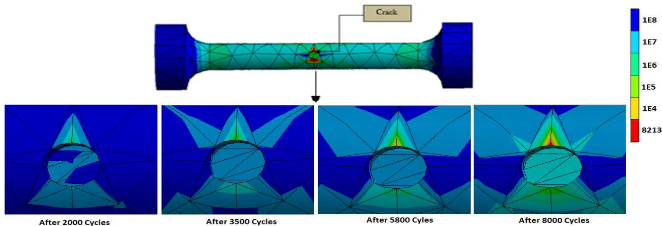
Figure 11 Fatigue behaviour of the cracked area during cyclic tests
