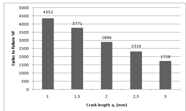
Fig 10. Crack length vs cycles to failure for different crack size
