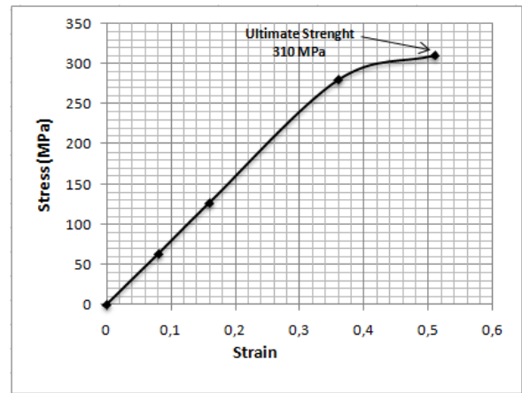
Fig 5 Stress-Strain curve
