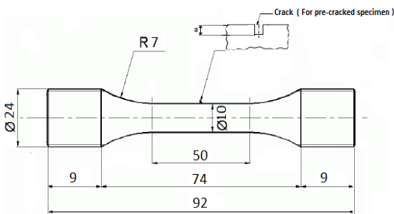
Fig 1 Specimens dimensions
