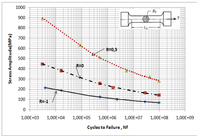
Fig 7 Comparison of the S-N curves under the three stress ratio
