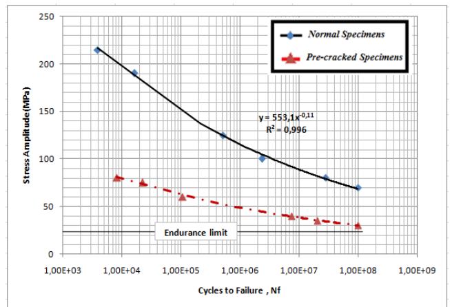
Fig 9 Comparison of S-N curves for the pre-cracked and normal specimen (R= -1, a=3mm)
