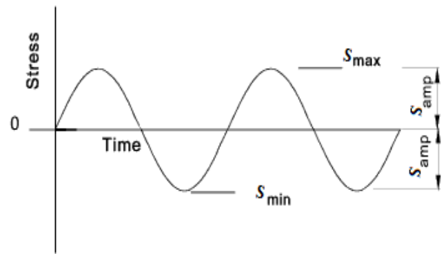
Fig 2..Applied Loading
