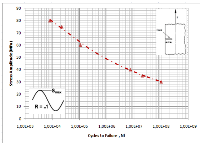
Fig 8 S-N curve for the pre-cracked specimen (crack length (a) =3mm and R= -1)
