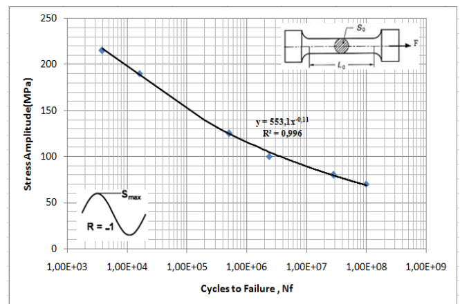
Fig 6. S-N curve under R = -1
