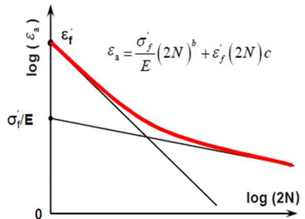
Fig.3. Strain-Life approach [20]
