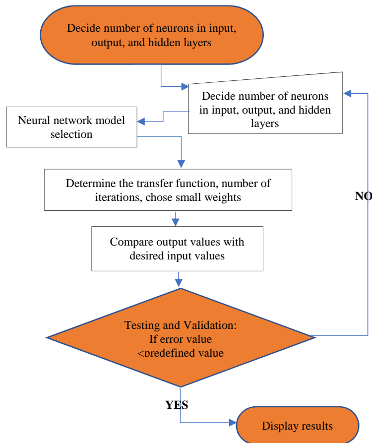
Fig. 2 Flowchart of process planning for prismatic part features based on LMBPNN
