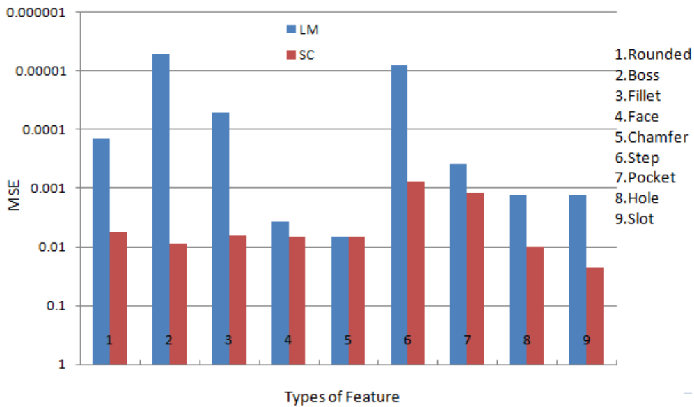
Fig .16 Comparison of LM and SC neural network
