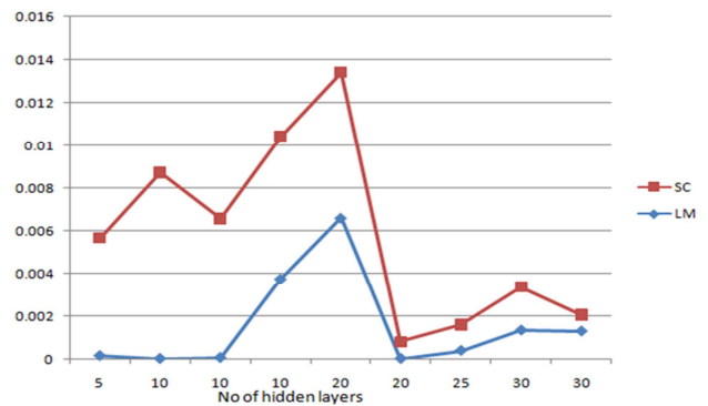
Fig .17 MSE for different hidden layers
