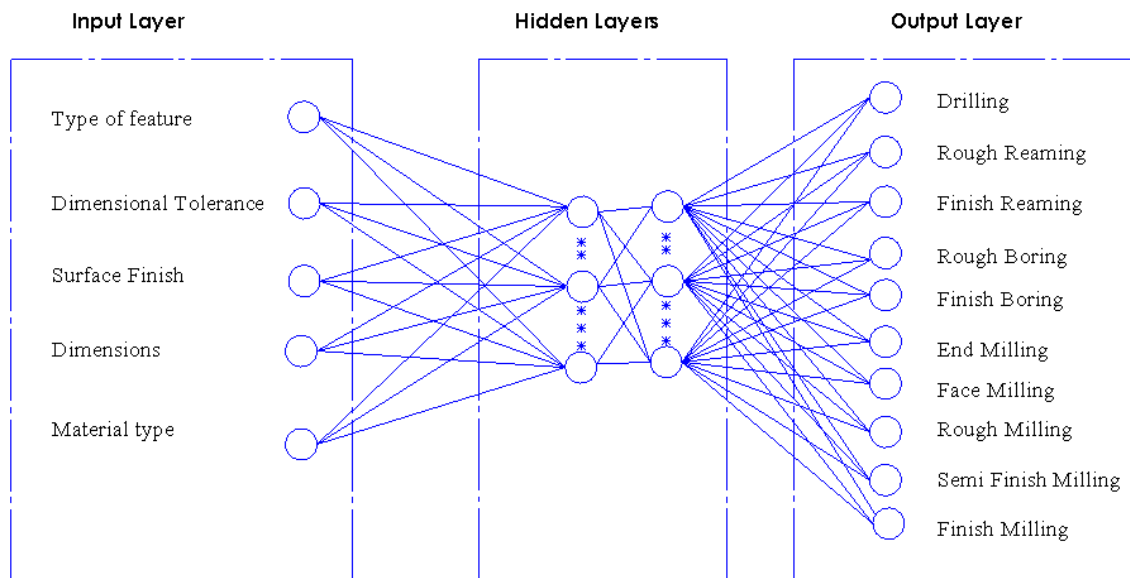
Fig.1 Machining operation selection
