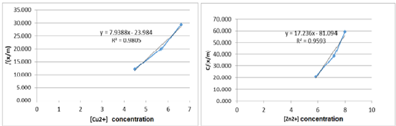
Fig. 4 Langmuir model fit for \text{Cu}^{2+} (left) and \text{Zn}^{2+} (right) adsorption by \text{HNO}_3 -activated cassava peels
