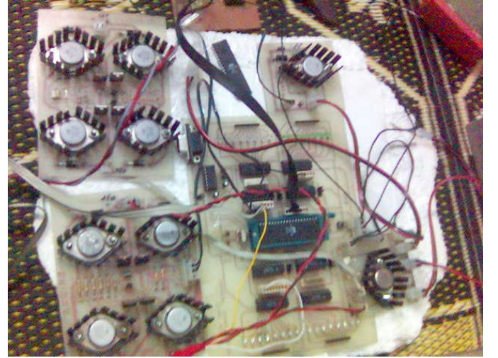
Fig. 5 Complete electronic circuitry of the PR robot manipulator
