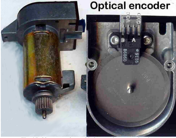
Fig. 6 Buhler motor along with the encoder mounted on it
