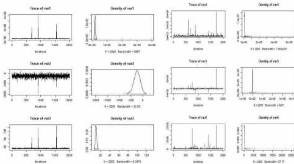
Figure 2: Trace and Posterior distribution
