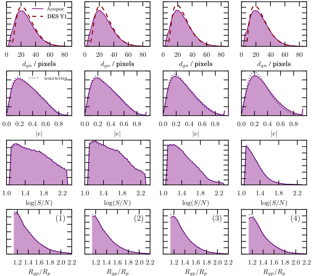
Figure 12. Measured histograms of observable properties in the main HOPOE and neighbour-free WAXWING simulations. The rows show (top to bottom) nearest neighbour distance, ellipticity, signal-to-noise ratio, and PSF normalized size. Each column (left to right) shows the distribution of galaxies in one of the four tomographic bins used in the DES Y1 cosmic shear analysis.
