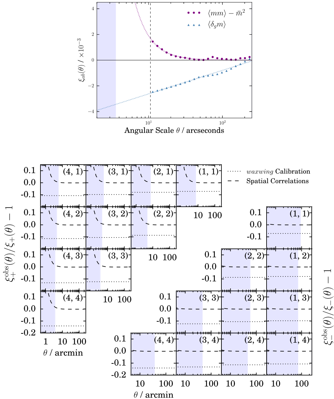
Figure 15. Top: The observed two-point correlation of multiplicative bias, as measured from the main HOOROE simulation set presented in this paper. Sub-patches are used to compute m in spatial patches of dimension 0.15 \times 0.15 deg and the correlation function calculated as described in the text. The dashed vertical line shows the diagonal scale of the sub-patches, below which we do not attempt to directly measure spatial correlations. The shaded blue bands show the minimum and maximum scales used in the DES Y1 cosmic shear analysis of Troxel et al. (2017). Bottom: Residuals between the mock two-point shear-shear data used in this paper, before and after different forms of bias have been applied. The upper-left and lower-right triangles show the \xi_+ and \xi_- correlations, respectively, calculated using the redshift distributions of Hoyle et al. (2017). The dotted black lines, which are flat across all scales but vary between panels, show the result of calibrating our Y1 shear measurements with a simple postage stamp simulation without image plane neighbours. The dashed lines illustrate the impact of ignoring scale-dependent selection effects, which are not captured by our simulation-based calibration. The shaded blue regions of each panel show the excluded scales for each particular tomographic bin pairing.
