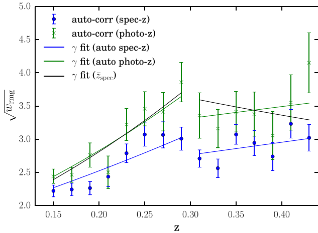
Figure 3. Integrated auto-correlations (equation (2)) of SDSS redMaGiC with spectroscopic redshift samples. Shown are the auto-correlations of the same sample but on either the spectroscopic or photometric redshift measurements. The auto-correlations on the photo-z measurements of redMaGiC samples use the correction of equation (9). We fit these auto-correlations in both Bin 1 ( z \in [0.15, 0.3] ) and Bin 2 ( z \in [0.3, 0.45] ) by (1+z)^\gamma in equation (7). The best fits are shown here, and their values are listed in Table 3. We note that although the spec-z and photo-z auto-correlations are offset in amplitude, our methodology (i.e. equation (6)) only depends on the redshift-dependence of the auto-correlations, parameterized by \gamma . The spec-z and photo-z auto-correlation fits are within \delta\gamma = 1 of each other.
