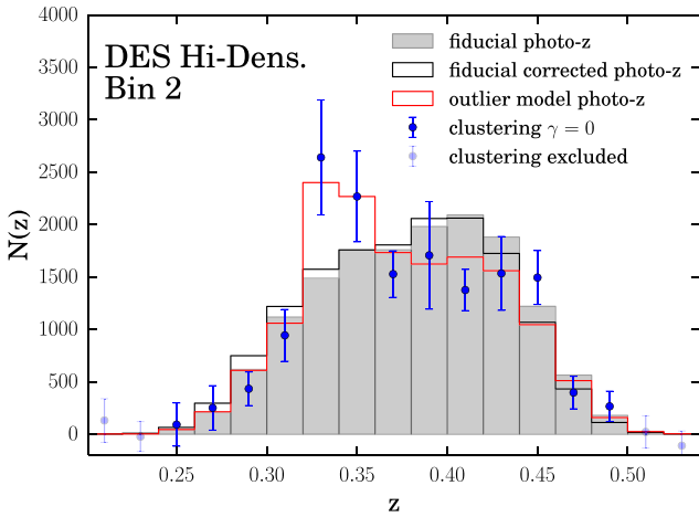
Figure 12. Comparison of the fiducial DES Y1 high-density redMaGiC Bin 2 ( z \in [0.3, 0.45] ) N(z) measurements, and shifted photo- z fit, to the outlier model described in Fig. 11. This improves the \chi^2/\text{dof} fit to 2.2 compared to 0.7 for the fiducial corrected photo- z fit of a single shift of \Delta z = 0.005 .
