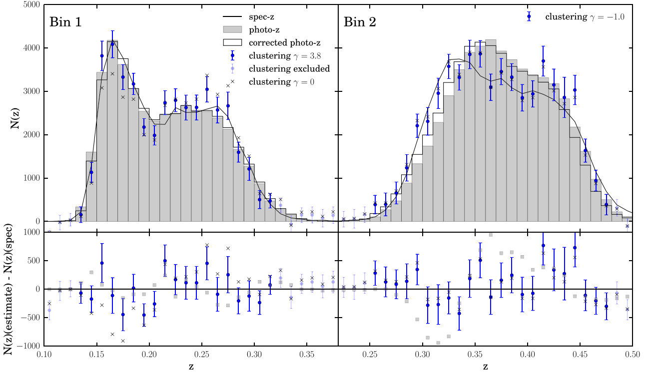
Figure 2. (Top row) SDSS redMaGiC with spectroscopic redshifts, high-density sample, clustering redshift distributions ( n_u(z) in equation (8)), photo-z distribution ( n_{pz}(z) in equation (10)), shifted photo-z fit ( n_{pz}(z + \Delta z) in equation (10)) and true spec-z distribution. The blue points have the values of \gamma that make the clustering estimate match the mean redshift of the spec-z (see Table 3). The black x's are the clustering estimate with \gamma = 0 (no bias correction). The 'clustering excluded' points are the clustering redshift estimates in the tails that are cut from analysis (see end of Section 3.2). (Bottom row) The residuals (number of galaxies) compare the clustering and photometric redshift distribution estimates with the spec-z distribution. The total residuals for the range where clustering is used are approximately for Bin 1: 5,400 for clustering, 2,700 for photo-z, Bin 2: 9,400 for clustering, 10,000 for photo-z.
