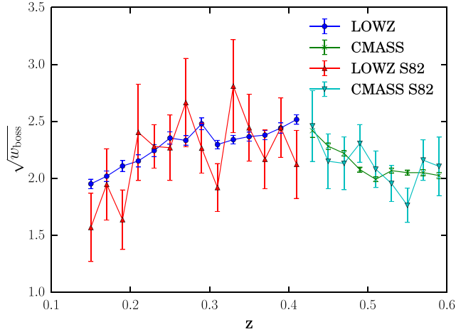
Figure 6. The square root of the integrated auto-correlation (equation (2)) of each of the reference samples from SDSS DR12, which is broken up into the LOWZ and CMASS surveys. The auto-correlations of the full sample are statistically consistent with the auto-correlations on the reference sample just within Stripe 82, but with less noise ( \chi^2/\text{dof} \leq 1 for both LOWZ and CMASS).
