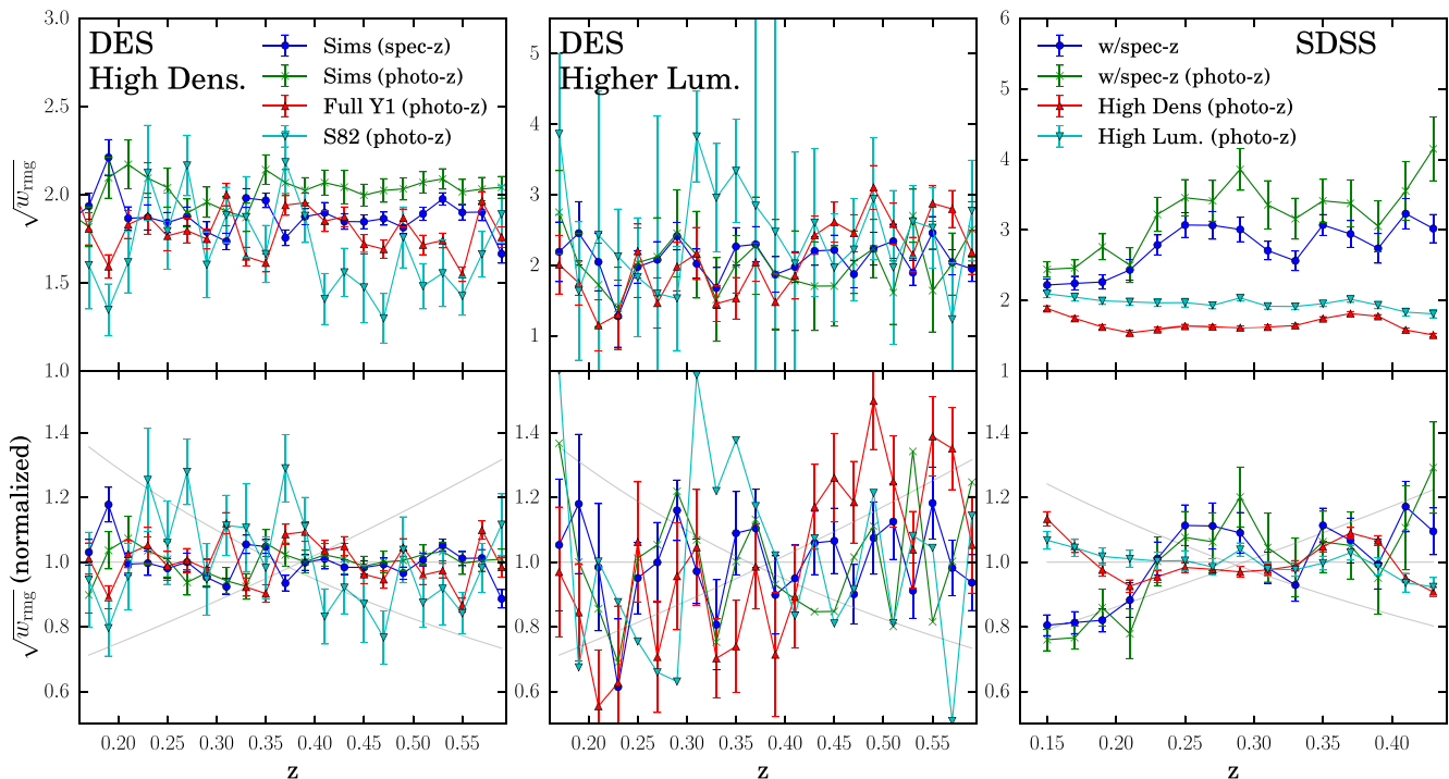
Figure 4. (Top row) Integrated auto-correlations (equation (2)) of DES and SDSS redMaGiC samples. The photo-z redMaGiC samples use the correction of equation (9). (Bottom row) The same auto-correlations normalized for better comparison between samples. Only the change in redshift matters as a systematic to the cross-correlation method, not the amplitude of the galaxy auto-correlation (equation (6)). We fit the normalized auto-correlations by (1+z)^\gamma in equation (7). Shown in grey are lines for (1+z)^\gamma with \gamma = -2, 0, 2 as examples, though we do fit across all possible values of \gamma . Each of the DES high-density samples and the SDSS high-density and high-luminosity samples are very consistent with \gamma = 0 . The DES higher-luminosity samples are much noisier due to fewer objects, so we also assume in our fiducial analysis \gamma = 0 \pm 2 . For the DES higher-luminosity sample, the full DES data set is closer to \gamma = 2 , though the simulations and Stripe 82 data agree with \gamma = 0 . In the normalized DES higher-luminosity plot, the error bars for the simulations (photo-z) and the Stripe 82 data have been removed for clarity since they span the entire y-axis range of the plot. Also shown in the right-hand panels again are the SDSS subsamples with spec-z measurements used in Section 4.1. Their significantly different bias evolution with redshift is apparent compared to the other redMaGiC samples (see Fig. 5 for more discussion on this).
