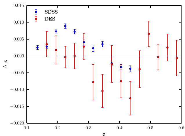
Figure 10. Comparison of the estimated photometric redshift bias for SDSS and DES high-density samples on dz = 0.03 size bins. The SDSS points are the same as in Fig. 9.
