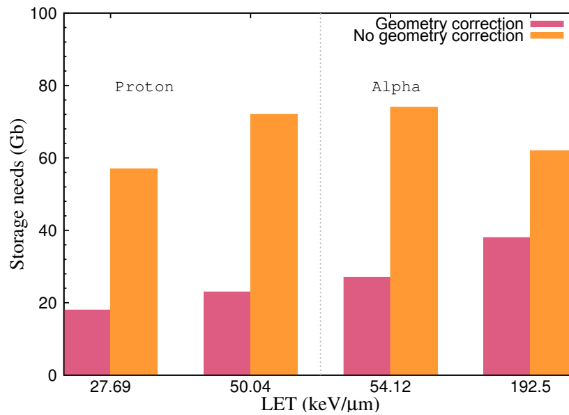
Figure 29 – Storage space occupied by the two protons (0.5 MeV and 1 MeV) and two alpha particles (2 MeV and 10 MeV). For each LET value the storage space is shown when the geometry correction is activated and when it is not used. The data for each particle is divided by a dotted line.
