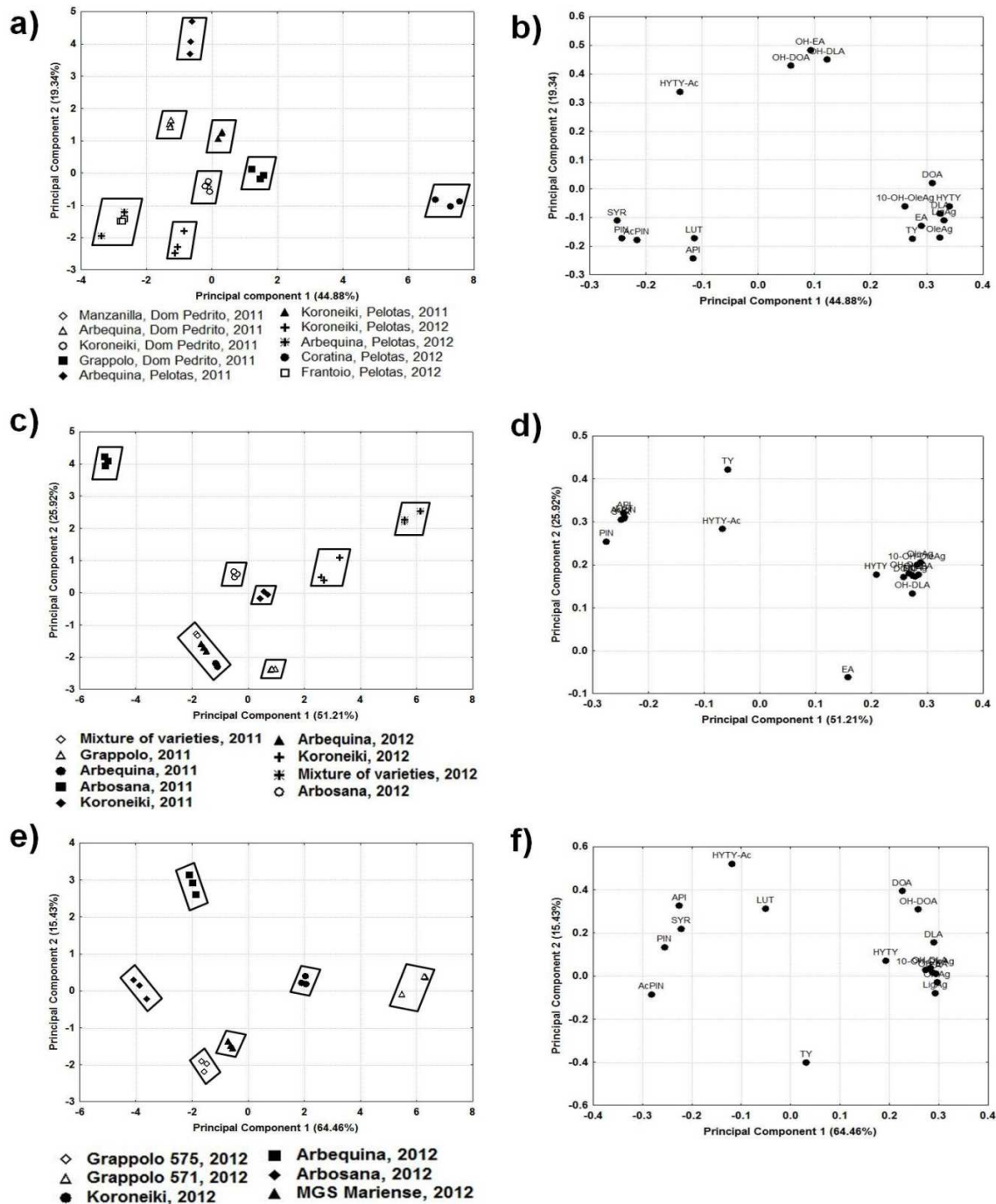
Figure 5.3. Results of the Principal Component Analysis, showing the first and the second principal components for the responses values. a) scores graph, Rio Grande do Sul state; b) loadings graph, Rio Grande do Sul state; c) scores graph, Santa Catarina state; d) Loadings graph, Santa Catarina state; e) scores graph, Minas Gerais state; f) loadings graph, Minas Gerais state.
