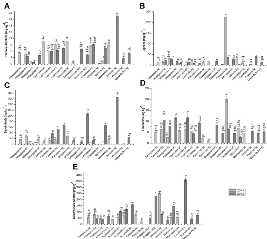
Figure 5.2. Phenolic alcohols (A), Lignans (B), Secoiridoids (C), Flavonoids (D) and Total Phenolic Contents (E), in mg kg -1 , of Brazilian extra-virgin olive oils. Columns followed by the same letters showed no significant difference ( p < 0.05 ) by the Tukey test. The letter between parenthesis after the variety name in the "x" axis refer to the place of origin: (a) Dom Pedrito, RS; (b) Pelotas, RS; (c) Chapecó, SC; (d), Maria da Fé, MG; (d1) Maria da Fé, MG, Grappolo 575; (d2) Maria da Fé, MG, Grappolo 541.
