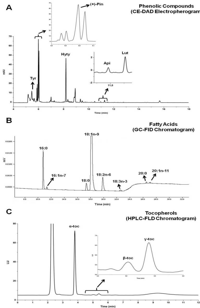
Figure 4.1. Representative electropherogram for the analysis of phenolic compounds ( A ), and representative chromatographic profiles for the analysis of fatty acids ( B ) and tocopherols ( C ) in Brazilian extra-virgin olive oil (Negroa variety, 2011 crop). Peak identification: Tyr, tyrosol; (+)-pin, (+)-pinoselinol; Hyty, hydroxytyrosol; Api, apigenin; Lut, luteolin; 16:0, palmitic acid; 16:1n-7, palmitoleic acid; 18:0, stearic acid; 18:1n-9, oleic acid; 18:2n-6, linolenic acid; 18:3n-3, \alpha -linolenic acid; 20:0, arachidic acid; 20:1n-11, 9-eicosenoic acid; \alpha -toc, \alpha -tocopherol; \beta -toc, \beta -tocopherol; \gamma -toc, \gamma -tocopherol.
