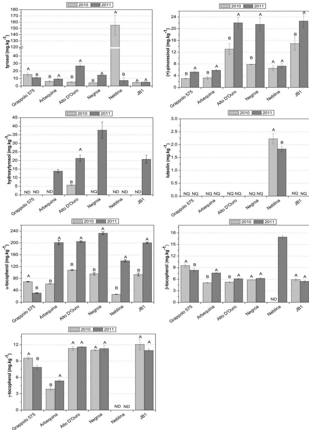
Figure 4.3. Comparison between the phenolic compound and tocopherol contents of Brazilian extra-virgin olive oil obtained from different varieties over two crop years. Bars followed by the same uppercase letters showed no significant difference ( p < 0.05 ) by the Tukey test, for the crop year comparisons.
