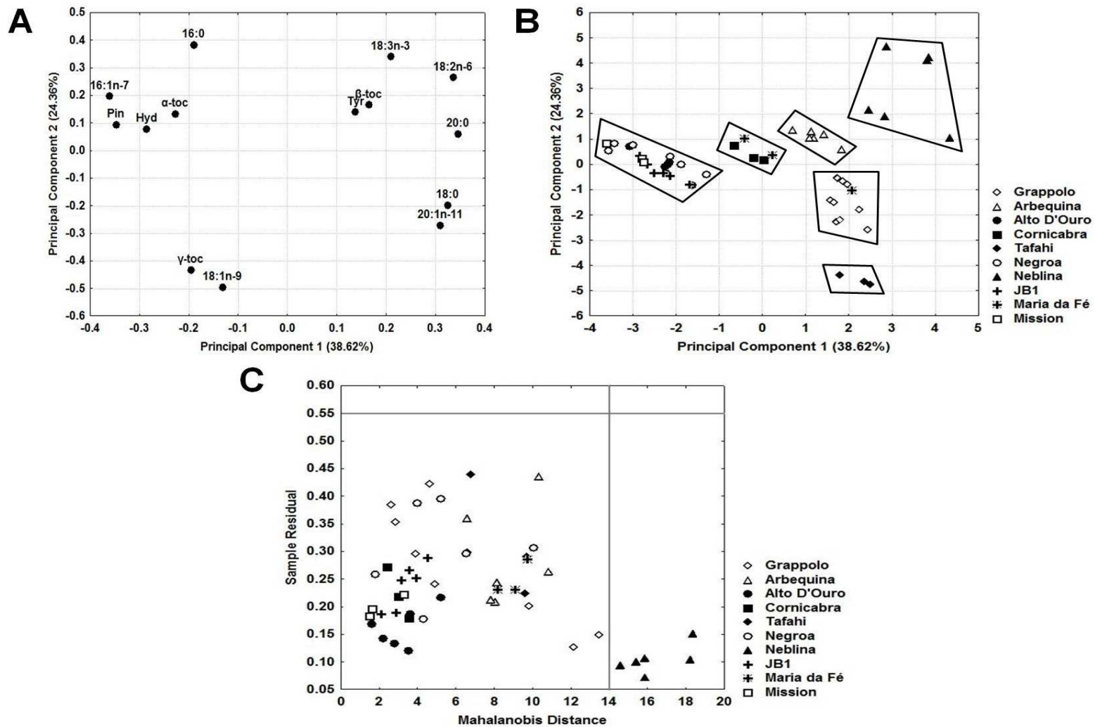
Figure 4.4. Results of the principal component analysis, showing the first and the second principal components for the response values. (A) Loadings graph; (B) Scores graph; (C) Mahalanobis distance graph.
