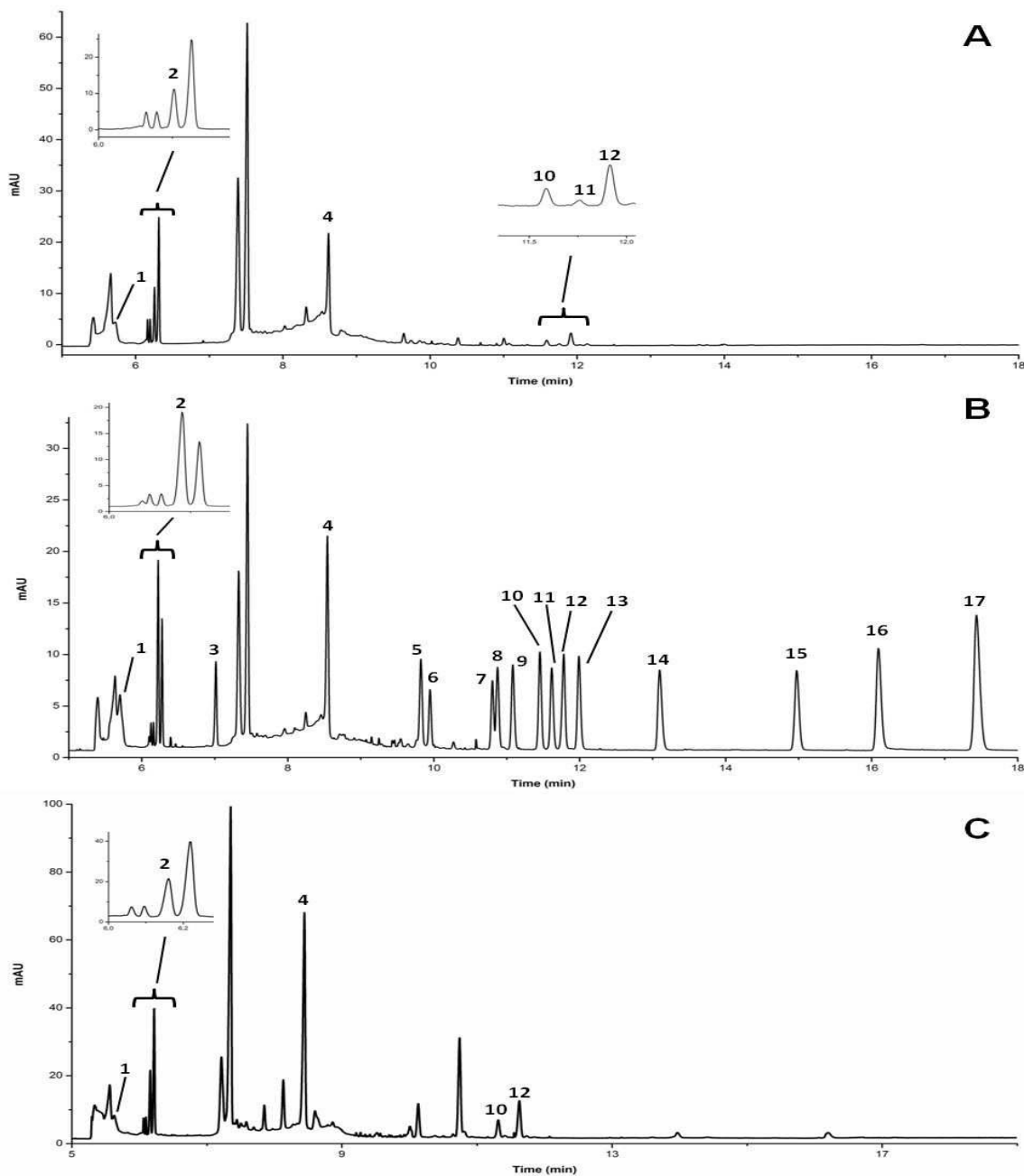
Figure 3.2. Representative electropherograms obtained for the polar extracts of the extra-virgin olive oil samples. A) Electropherogram for the polar extract of sample n° 1. B) Electropherogram for the polar extract of sample n° 1 spiked with the seventeen phenolic compound standards. C) Electropherogram for the polar extract of sample n° 15. Some regions of the electropherograms were enlarged to better visualize some of the compounds detected in the samples. Electrophoretic conditions and peak identification can be seen in Figure 3.1 .
