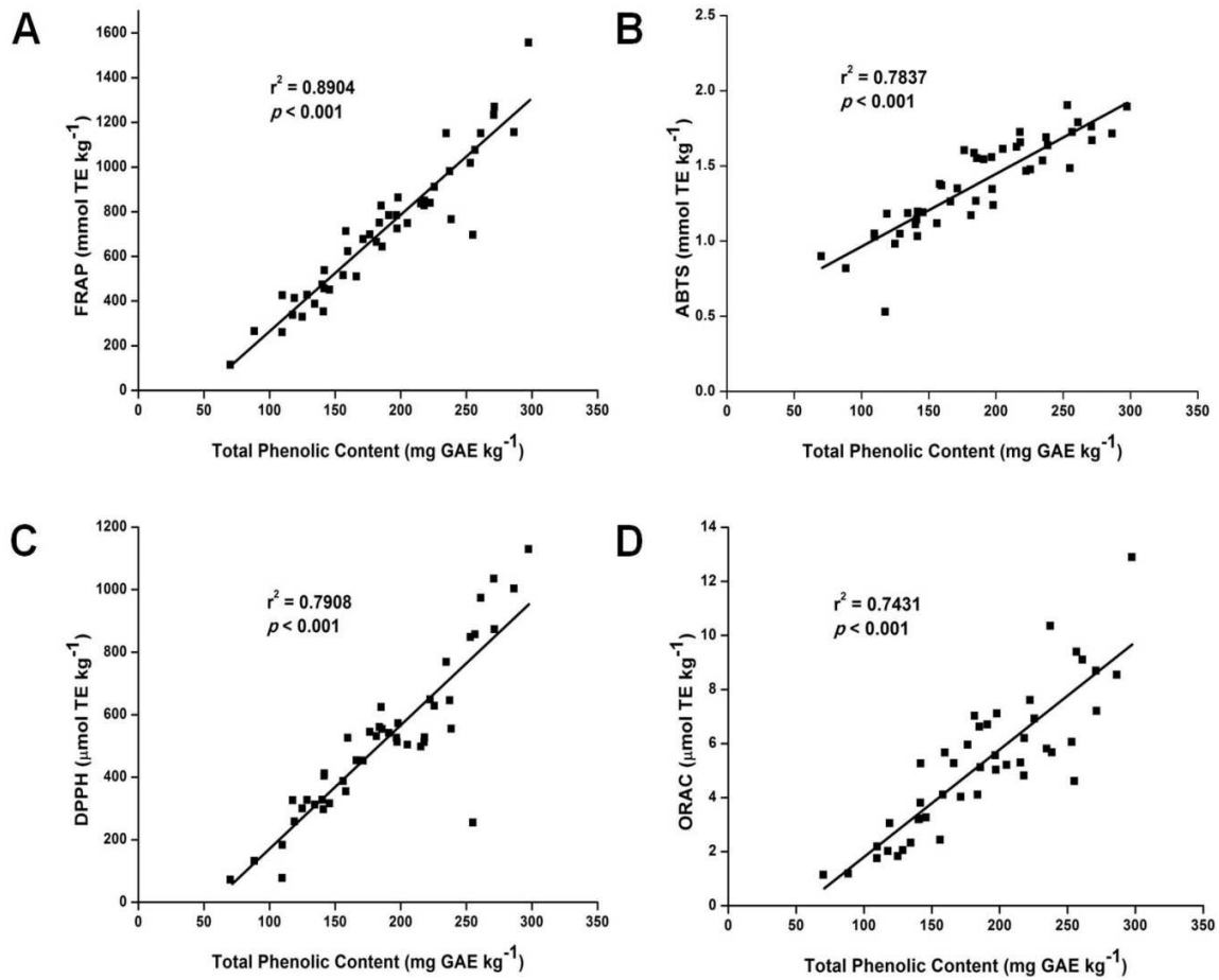
Figure 2.2. Correlation between the total phenolic content and each one of the four antioxidant capacities of the extra-virgin olive oil samples. A) FRAP assay; B) ABTS assay; C) DPPH • assay; D) ORAC assay.
