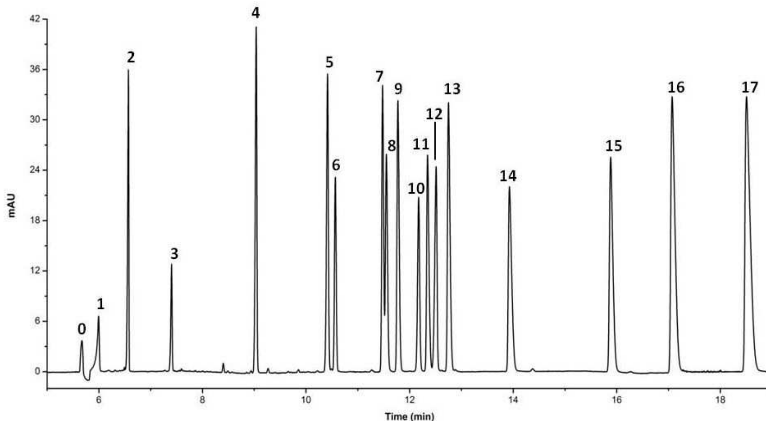
Figure 3.1. Electropherogram for the optimal separation of seventeen phenolic compounds. Fused-silica capillary of 50 \mu\text{m} internal diameter and 72 cm of effective length with extended light path, 101.3 \text{mmol}\cdot\text{L}^{-1} of boric acid electrolyte at 9.15 pH, 30 kV, 25°C, injection of 0.5 Pa for 5 seconds, and detection at 210 nm. Peak identification: 0, solvent; 1, tyrosol; 2, (+)-pinoresinol; 3, oleuropein glycoside; 4, hydroxytyrosol; 5, cinnamic acid; 6, sinapinic acid; 7, syringic acid; 8, ferulic acid; 9, o -coumaric acid; 10, apigenin; 11, p -coumaric acid; 12, luteolin; 13, vanillic acid; 14, p -hydroxybenzoic acid; 15, caffeic acid; 16, gallic acid; 17, 3,4-dihydroxybenzoic acid.
