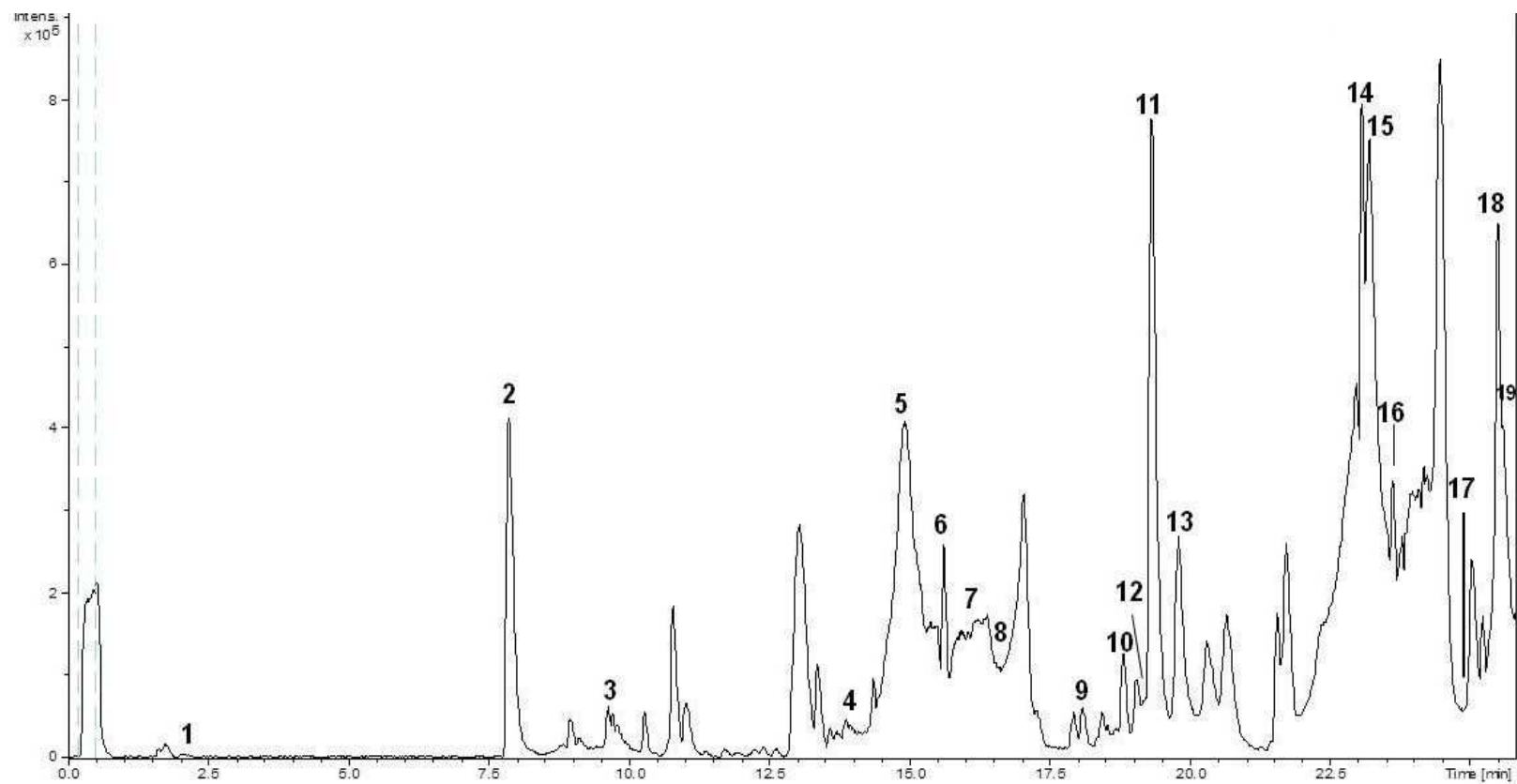
Figure 5.1. Base-peak chromatogram (BPC) of a representative Grappolo (Dom Pedrito, RS, 2011 crop) EVOO polar extract, obtained by RRLC-ESI-TOF-MS. Peak identification is the same as provided in Table 5.2 .
