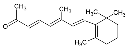
\beta -APO-13-CAROTENONE
