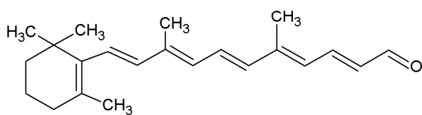
\beta -APO-14-CAROTENAL
