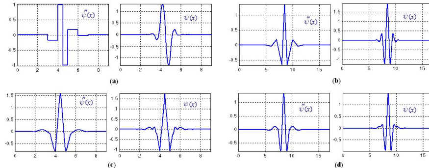
Figura 7.3: Wavelets Biortogonais \psi(x) e suas duais \tilde{\psi}(x) : (a) bior1.5; (b) bior2.8; (c) bior4.4; (d) bior6.8.
