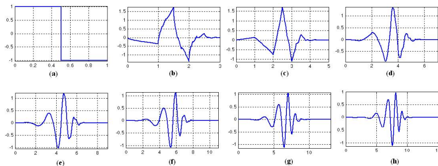
Figura 7.1: Wavelets de Daubechies para: (a)N=1; (b)N=2; (c)N=3; (d)N=4; (e)N=5; (f)N=6; (g)N=7; (h)N=8.
