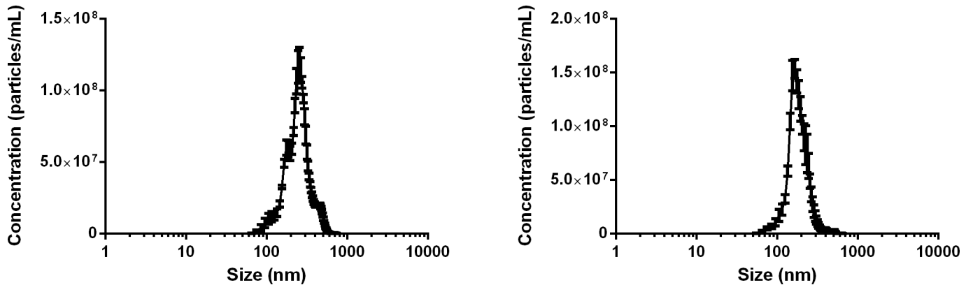
Fig 2. Nanoparticle concentration as a function of particle size (nm). (a) SLN and (b) 15d-PGJ 2 -SLN performed at 25°C (n = 5).
