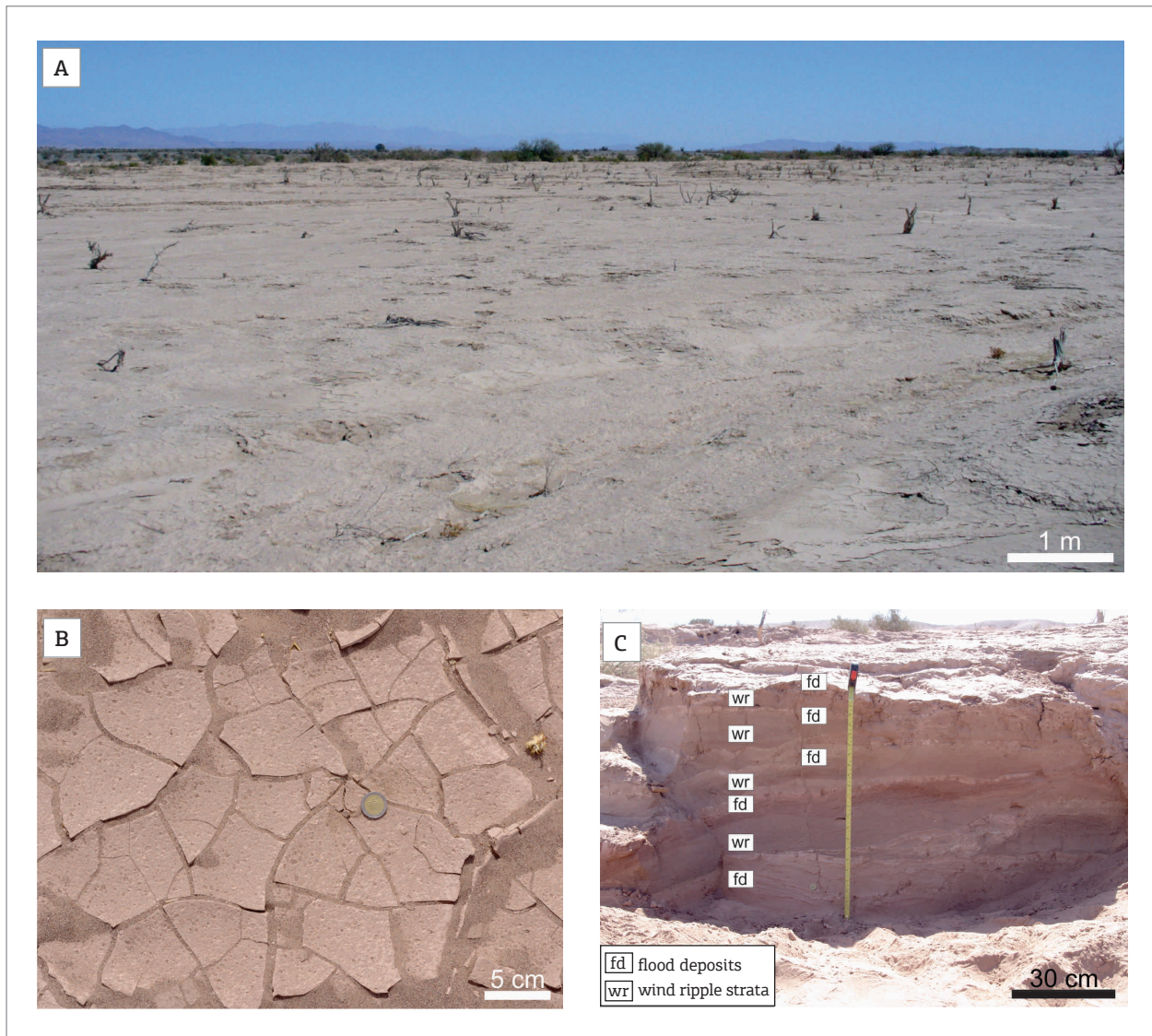
Figure 12. Flood deposits. (A) Irregular and newly formed depositional surface after rainwater flooding. (B) Desiccation cracks filled with eolian sand. (C) Natural exposure showing the vertical interbedding of flood deposits and wind ripple strata.
