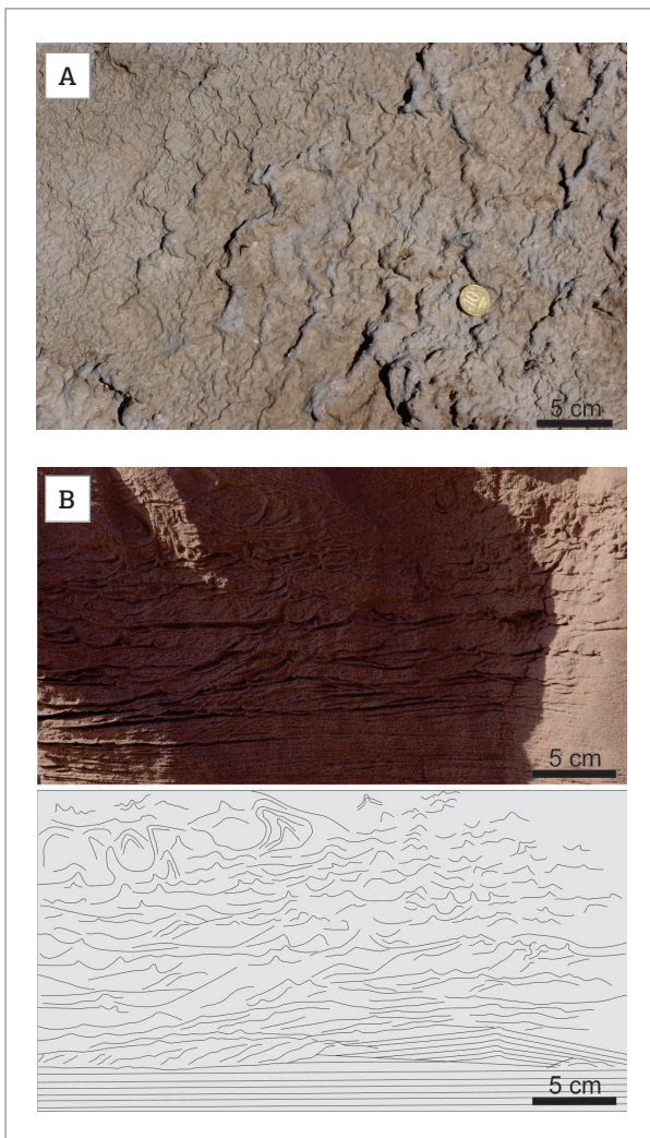
Figure 10. Damp eolian features. (A) Evaporitic-adhesion structure in plain view. The topographic surface is wrinkled and shows the bicolored pattern typical of this structure. (B) Small-scale deformation on wind ripple deposits. Contortion and disruption of the laminae evidence liquefaction at or close to the depositional surface.
