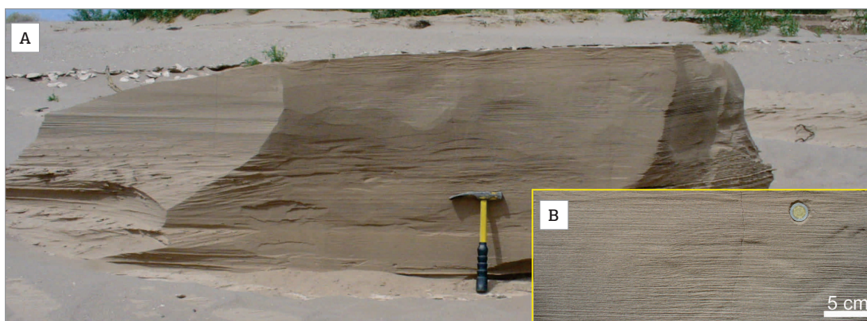
Figure 8. Yardang. (A) Wind-sculptured micro-yardang form developed on wind ripple deposits. (B) Detail of the deposits showing very fine- to fine-grained sandstone with inversely graded wind ripple strata. The hammer is 0.34 m long.
