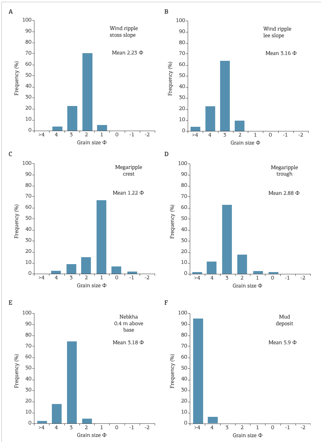
Figure 5. Grain size data.
