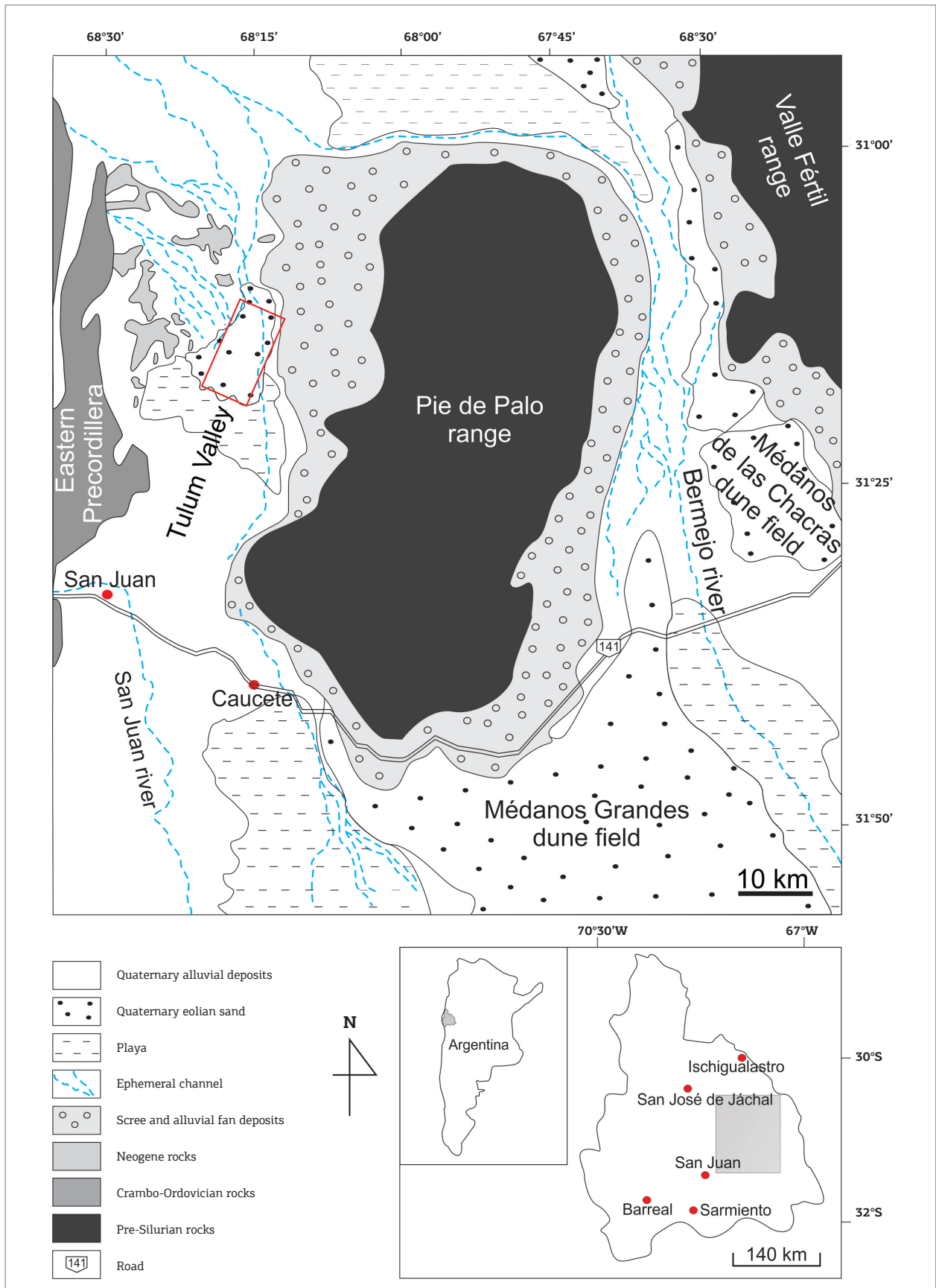
Figure 1. Geologic and geomorphologic map of the Tulum Valley. The rectangle delimits the study area.
