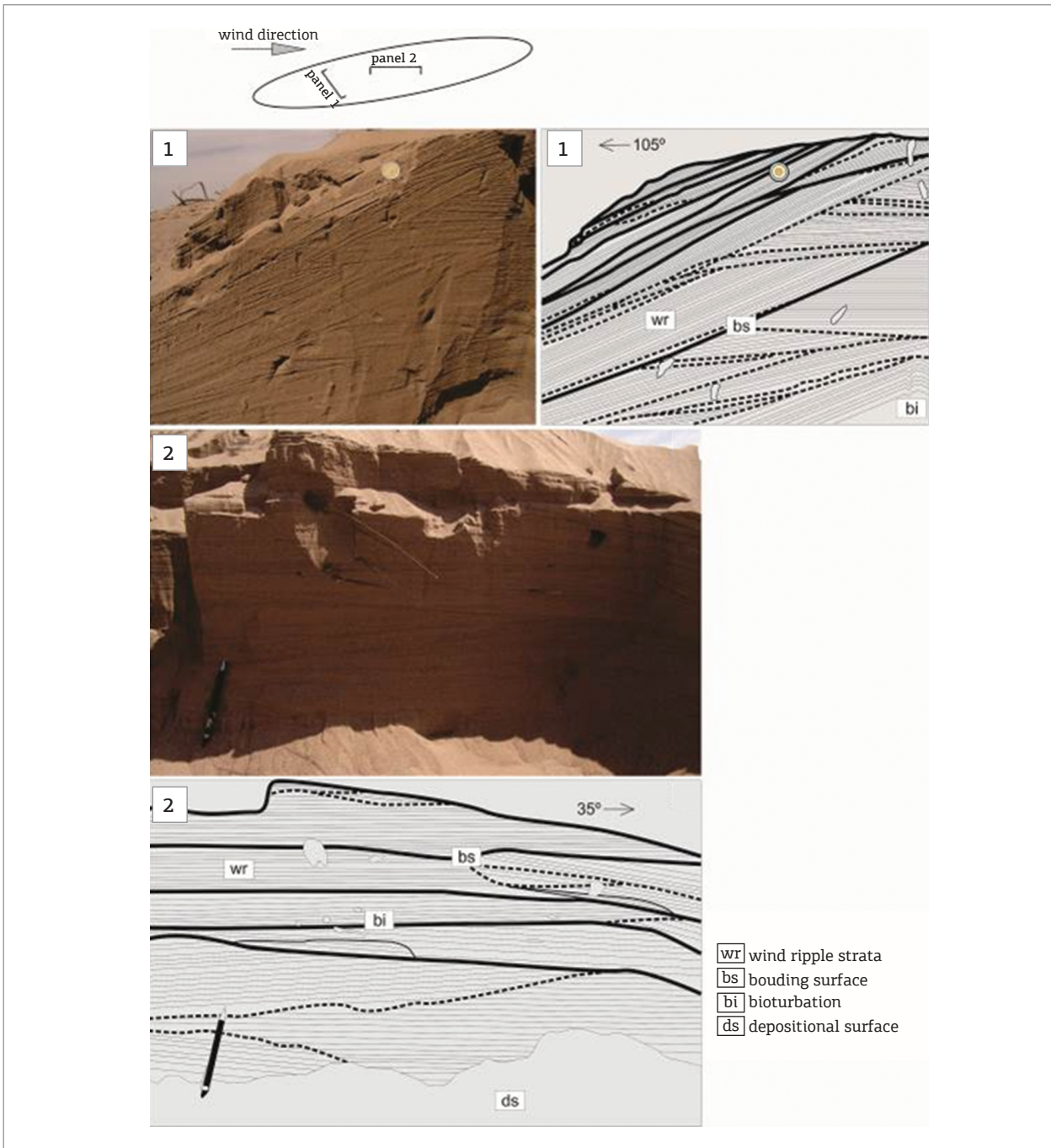
Figure 9. Internal sedimentary architecture of a nebkha. Panel 1 is oriented perpendicular to the wind direction and panel 2 is oriented parallel to the wind direction. Solid lines represent major bounding surfaces and dashed lines, minor bounding surfaces. The coin for scale is 20 mm in diameter, and the pencil is 0.14 m long.
