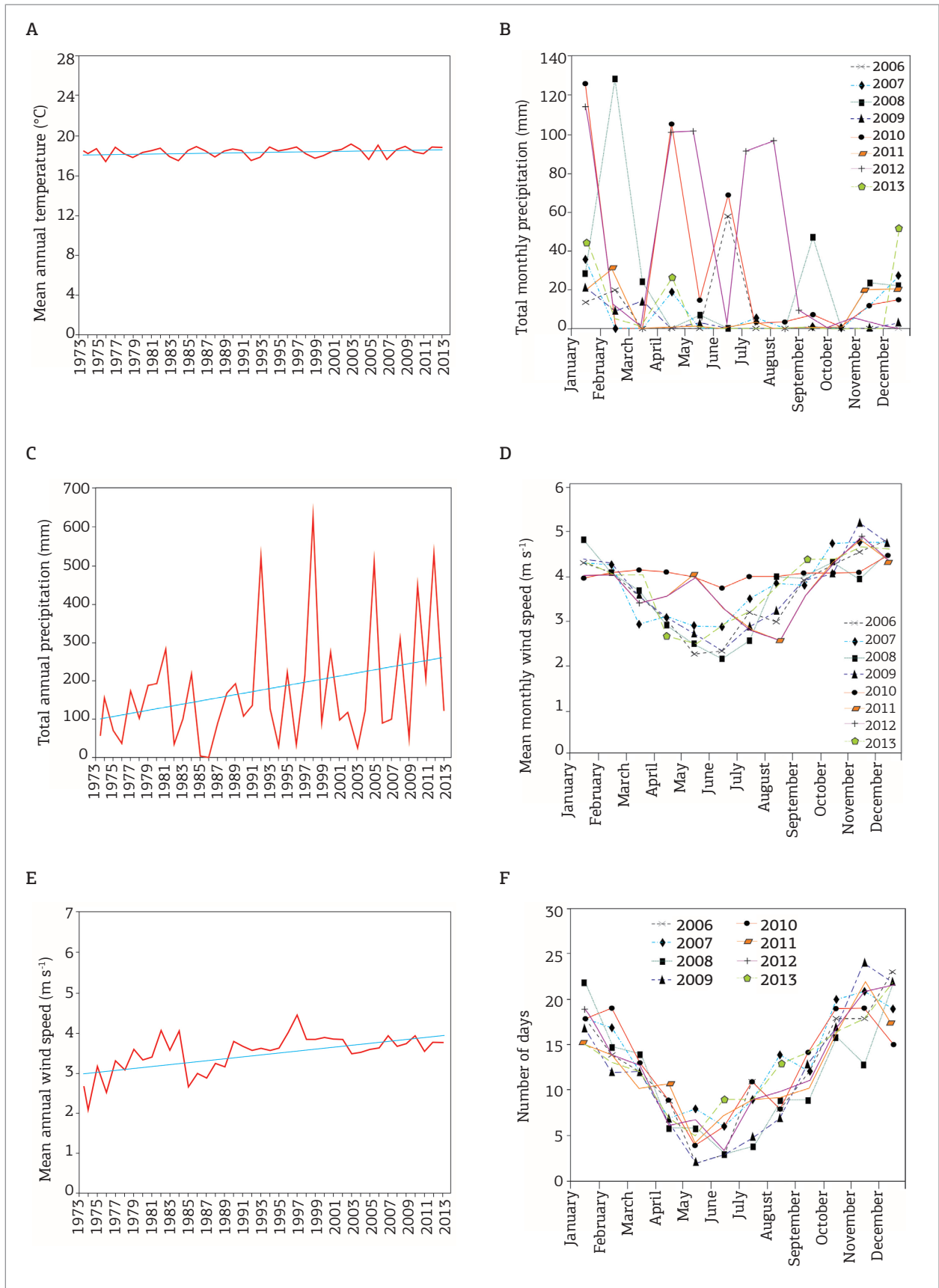
Figure 3. Summary climatic data for the San Juan region (data from weather station San Juan Aero: 31°34'S; 68°41'W).
