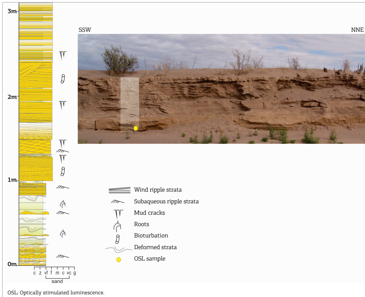
Figure 13. Stratigraphic section measured in the central part of the sand sheet showing the vertical interbedding of eolian and subaqueous deposits.
