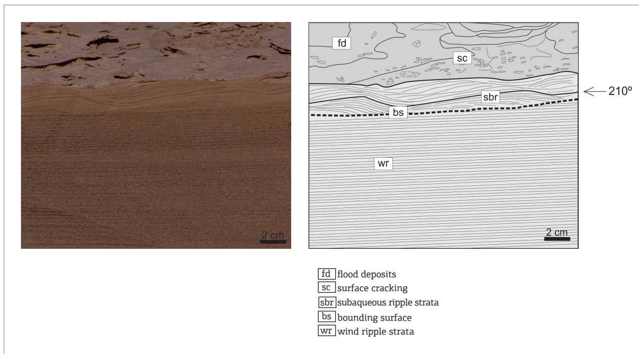
Figure 11. Subaqueous sedimentary features showing the vertical transition from wind ripple strata to subaqueous ripple strata which are overlain by silty mud deposits.
