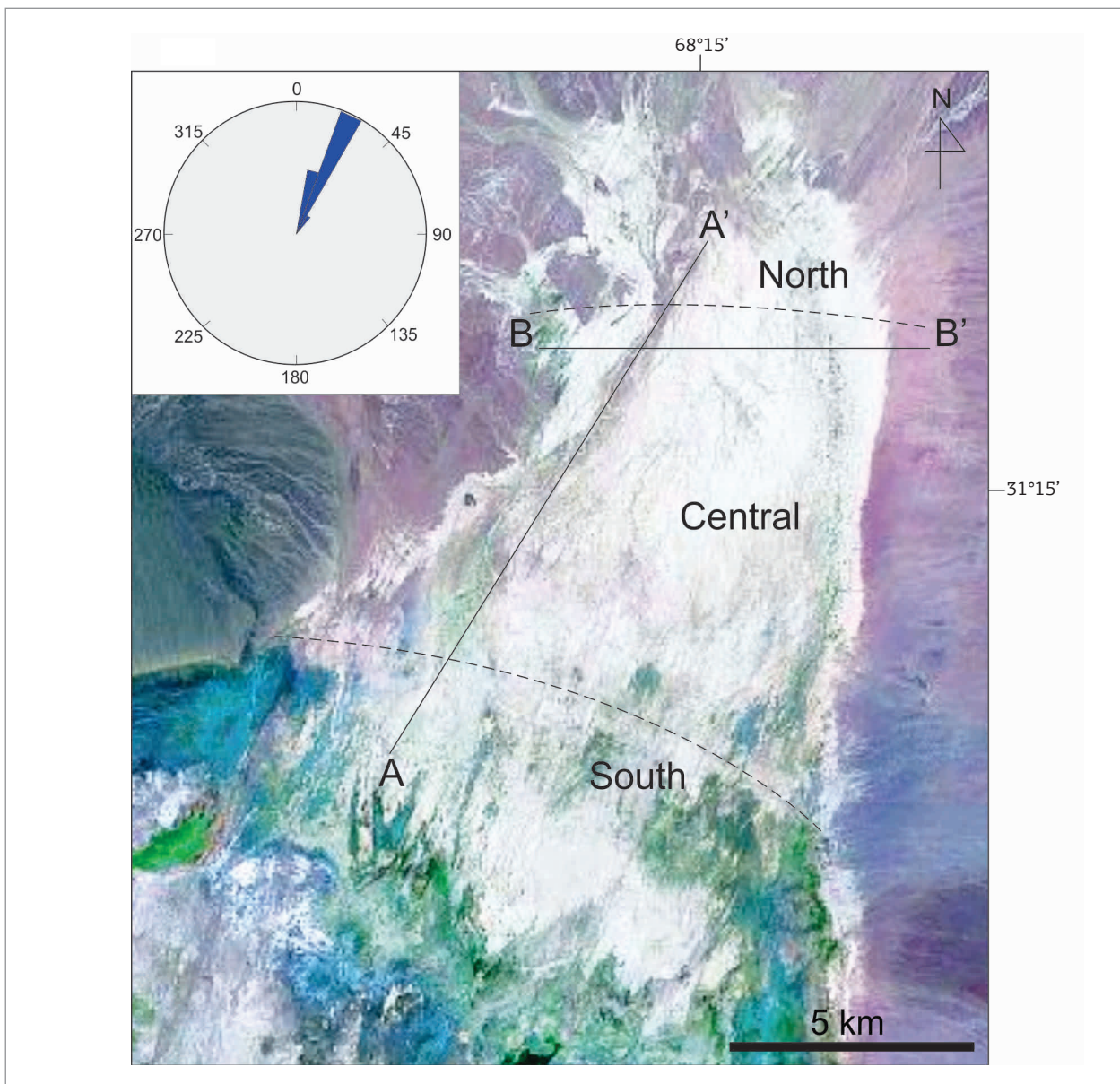
Figure 4. Landsat ETM+ image (bands 7, 4 and 2) of the intermontane Upper Tulum eolian sand sheet. The transect A-A' follows the main dry channel of the study area and the transect B-B' cuts transversally the dry channel section. The sand sheet compartmentalization into south, central, and north regions follows A-A' transect. Wind rose diagram (on the upper left corner) was constructed from measured sedimentary structures and indicates sediment transport towards northeast.
