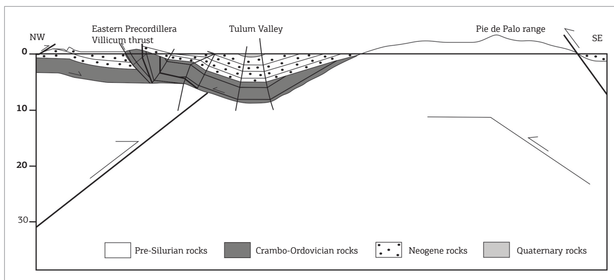
Figure 2. Schematic SE-NW crustal-scale regional profile from Pie de Palo range (southeast) through intermontane Tulum Valley to eastern Precordillera (northwest). Modified from Meigs et al. (2006).
