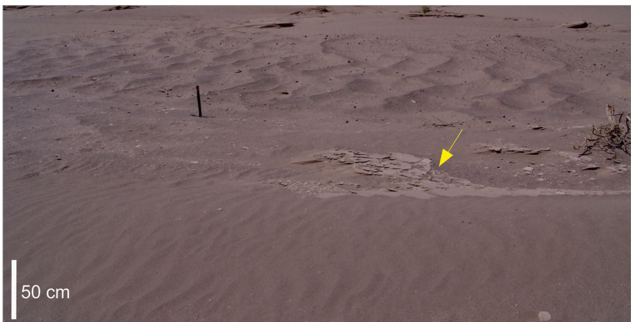
Figure 6. Oblique view showing wind ripples in the foreground and megaripples in the background. The arrow shows a thin layer of mud deposits.
