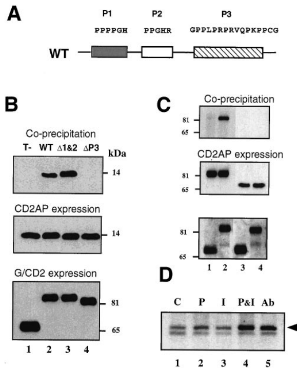
Figure 5. Mapping the Interaction between CD2AP and CD2 (A) Schematic diagram of VSV-G-CD2 constructs used to map the interaction between SH3-1 of CD2AP with murine CD2. The proline-rich sequences are represented by the gray and open boxes. (B) CD2AP binds to a proline-rich region at the C terminus of the CD2 cytoplasmic domain. The first CD2AP SH3 domain was appended with the myc epitope and coexpressed with VSV-G/CD2 constructs lacking either P1 and P2 or the P3 proline sequences using the vaccinia-T7 expression system in HeLa cells. VSV-G constructs were immunoprecipitated, separated by SDS-PAGE, transferred, and blotted with anti-myc followed by a secondary HRP-conjugated antibody, and developed using chemiluminescence. Immunoblotting of cell lysates to control for expression of myc-CD2AP (middle panel) and VSV G (lower panel) are shown. (C) Only the first SH3 domain of CD2AP binds to CD2. The VSV G/CD2 chimera (lanes 2 and 4) was coexpressed with either full-length myc-CD2AP (lanes 1 and 2) or with a myc-CD2AP construct lacking the first SH3 domain (lanes 3 and 4). A VSV-G tail minus construct, T- (lanes 1 and 3), was used as a control. The VSV-G immunoprecipitates were separated by SDS-PAGE and immunoblotted following transfer to nitrocellulose using a monoclonal antibody to the myc epitope tag. The proteins were visualized using a secondary HRP-conjugated antibody and chemiluminescence. Expression controls for myc-CD2AP (middle panel) and for VSV G (lower panel) are shown. (D) Activation-dependent association between CD2 and CD2AP in Jurkat T cells. Jurkat T cells were treated with PMA (P), Ionomycin (I), PMA + Ionomycin (P&I), with an activating pair of CD2 antibodies (Ab), or left untreated (C). Cells were lysed and immunoprecipitates prepared with antibodies to CD2, separated by SDS-PAGE, transferred to nitrocellulose, and developed with polyclonal antibodies to CD2AP.
