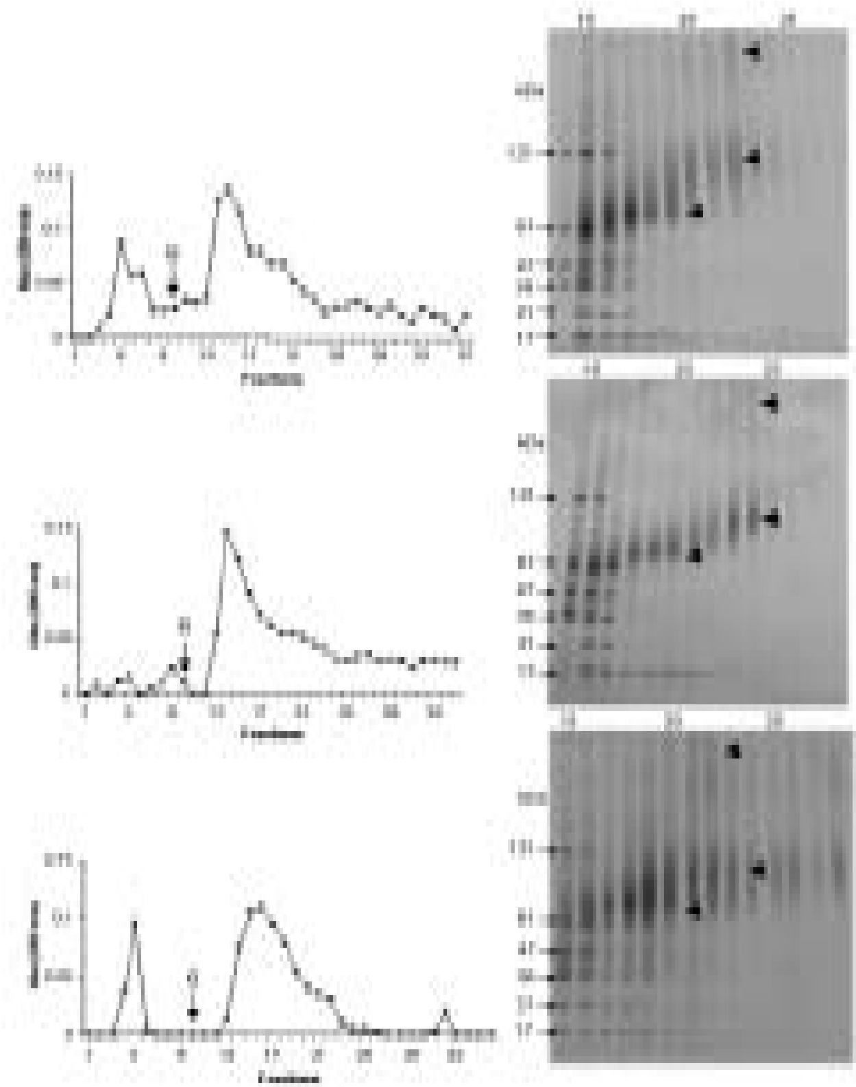
FIGURE 3. DEAE-Sephacel chromatography (A,C,E) and SDS-PAGE (B,D,F) of PL, PM and DC extracts. The proteins were eluted with a gradient (0.1-1.0 M) of NaCl. G - start of the gradient. The gels show proteins with molecular masses 121, 61, 47, 36, 21 and 17 kDa. Polydisperse bands were also seen at 67, 80-100 and 250-300 kDa ( ). ω
