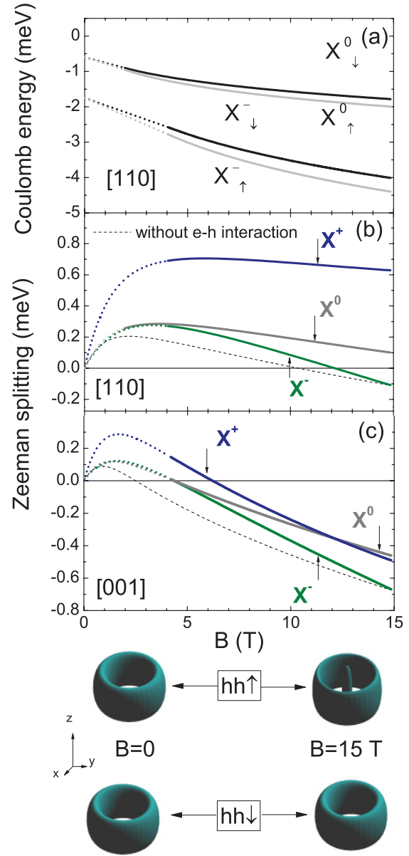
FIG. 1. (Color online) (a) Calculated Coulomb contribution to neutral exciton X^0 and trion X^- (ground state) binding energies vs magnetic field in a 23 nm (110) QW for two spin configurations indicated by vertical arrows. The dotted lines indicate the extrapolation of the Coulomb energy for zero magnetic field where the perturbation theory fails. (b) Calculated Zeeman splitting for optical recombination of X^0 and X^\pm excitonic complexes in the (110) QW. The dotted lines correspond to the Zeeman splitting considering the extrapolated Coulomb energy. The dashed line curve shows the splitting for X^0 without Coulomb interaction. (c) Calculated Zeeman splitting for optical recombination of X^0 and X^\pm excitonic complexes in a (001) QW. The lower panel shows the orbital shape for the hh \uparrow hh \downarrow states with z component of the angular momentum m = 2 at magnetic fields B = 0 and B = 15 T.
