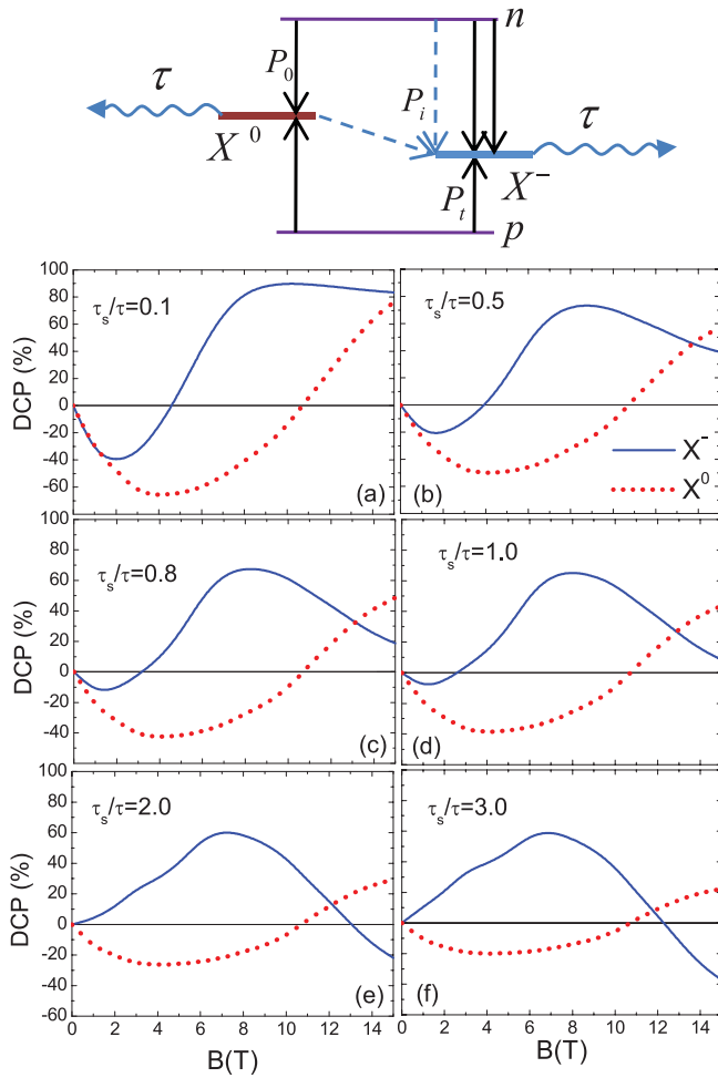
FIG. 6. (Color online) Upper panel: diagram representing the combined exciton and trion dynamics at B = 0 considered in the numerical simulations. (a)–(f) Theoretical calculations of the DCP for the neutral exciton, X^0 (dotted curves), and the trion, X^- (solid curves), as functions of the magnetic field by varying the parameter \tau_s/\tau within the range [0.1,3.0].
