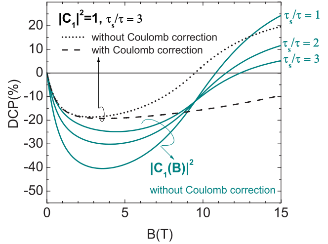
FIG. 5. (Color online) Theoretical calculations of the degree of circular polarization for the neutral exciton, X^0 : dotted and dashed curves, without considering the valence band hybridization, and solid curves (considering the valence band hybridization tuning with magnetic field varying the parameter \tau_s/\tau within the range [1.0,3.0]).
