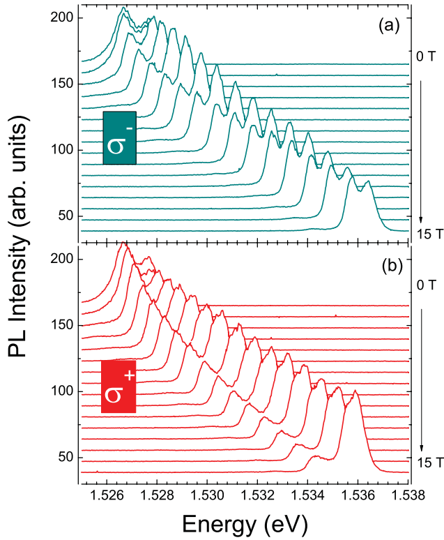
FIG. 3. (Color online) Magnetophotoluminescence spectra for different values of the magnetic field at T = 2 K and for excitation power of 5 nW: (a) for \sigma^- and (b) for \sigma^+ polarized emissions.
