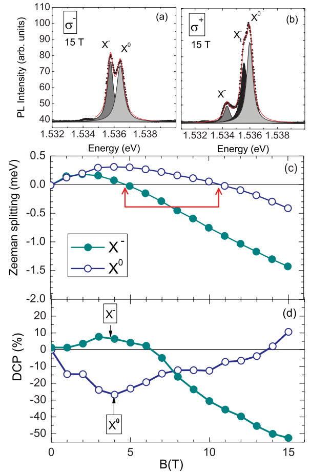
FIG. 4. (Color online) Spectral analysis of the magnetophotoluminescence spectra at B = 15 T for: (a) \sigma^- emissions and (b) \sigma^+ emissions. (c) Zeeman splitting of X^0 and X^- complexes as a function of the applied magnetic field extracted from the spectral analysis of the circularly polarized emissions. The critical magnetic field values where spin-inversion occurs are indicated. (d) Degree of circular polarization extracted from the PL spectra: open and filled circles correspond to the polarization of X^0 and X^- complexes, respectively.
