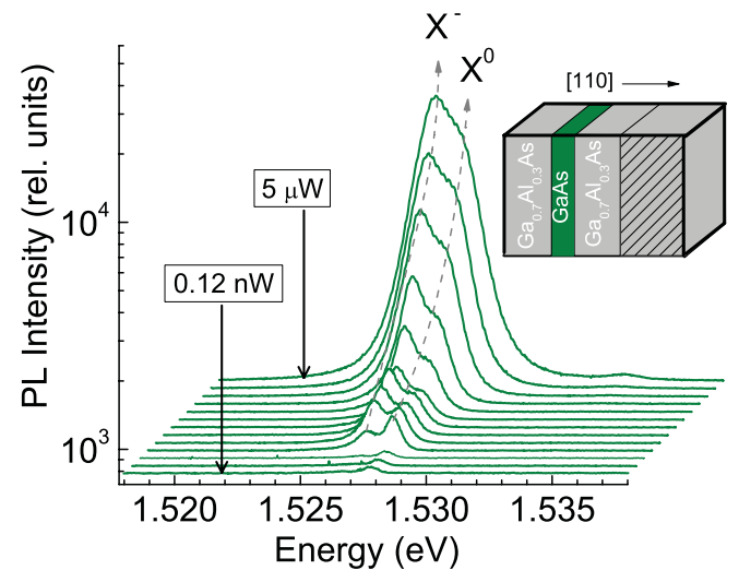
FIG. 2. (Color online) Magnetophotoluminescence taken at T = 2 K for excitation power ranging from 0.12 nW to 5 \mu W. The enhancement of the lower-lying emission line with increasing power is ascribed to an increasing density of negatively charged trions ( X^- ) and, consequently, the decreasing numbers of neutral excitons ( X^0 ). The inset illustrates the structure of the GaAs/AlGaAs (110) QWs.
