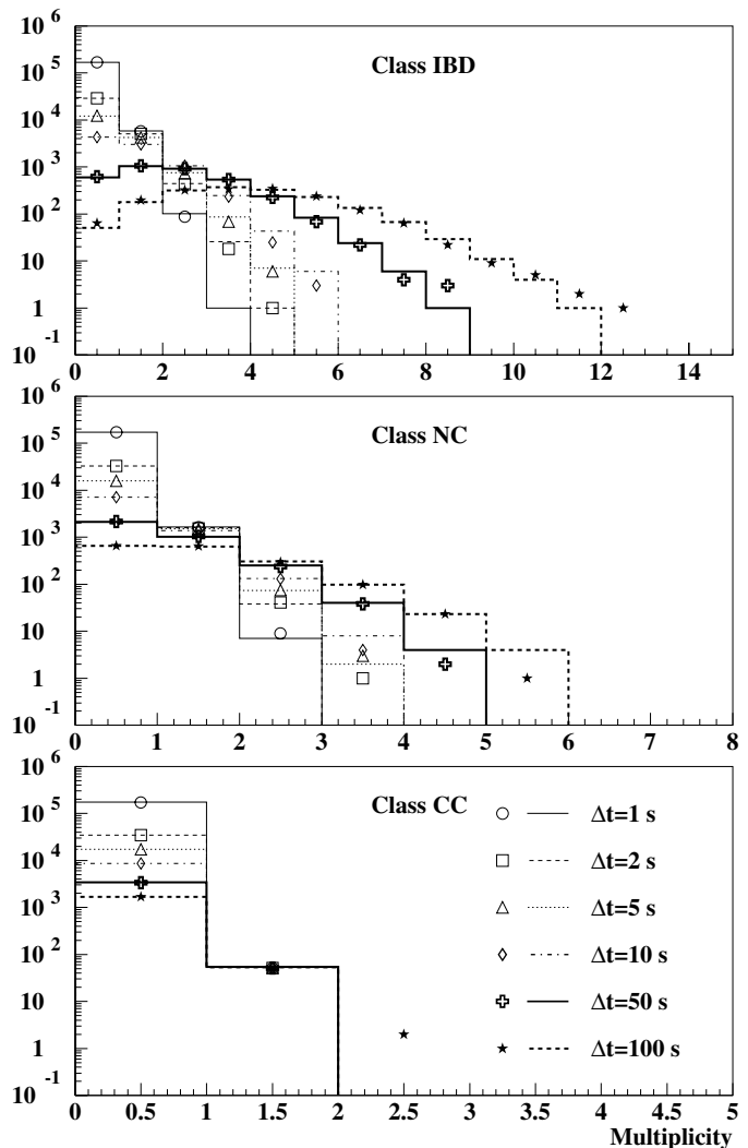
Fig. 2. Distributions of cluster multiplicities, for IBD class events (top), NC class (middle), CC class (bottom), together with expectations from Poissonian fluctuations, in the case of GW event n.5 .
