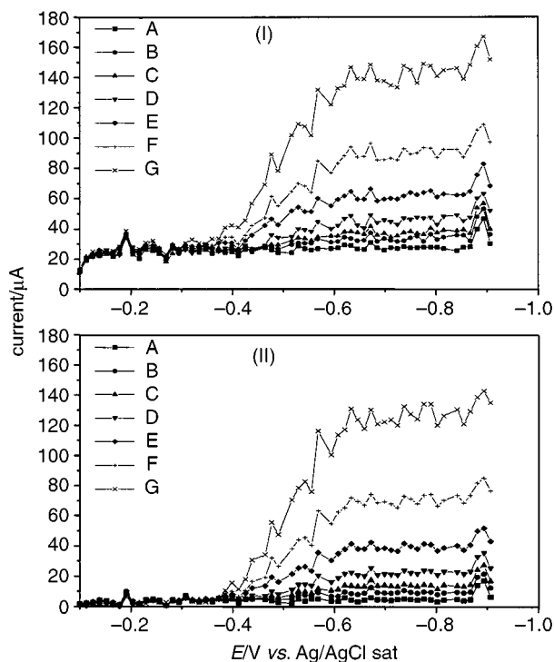
Fig. 3 Pseudo-voltammetric curves obtained by the multiplexed technique showing the behaviour of the faradaic current as function of the concentration of lead in 0.1 \text{mol L}^{-1} \text{NaNO}_3 solution [A, blank; B–G, 24 , 48 , 95 , 186 , 358 , 666 \mu\text{mol L}^{-1} \text{Pb(II)} , respectively]. Pseudo-voltammetric curves obtained by (I) electrode scan and (II) multiplexed scan.
