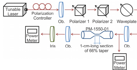
Fig. 4. Optical characterization setup. Ob.: objective lens.
