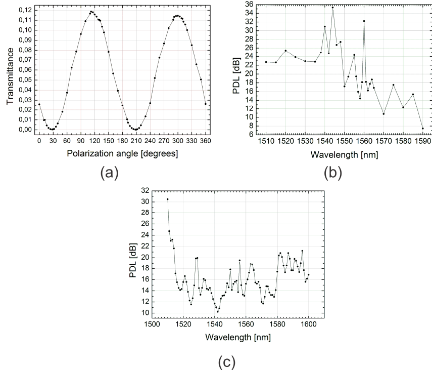
Fig. 5. (a) Fiber transmittance as a function of input polarization angle at 1560 nm. Measured PDL spectra in the 1510-1600 nm range for tapered PCF samples 1 (b) and 2 (c).
