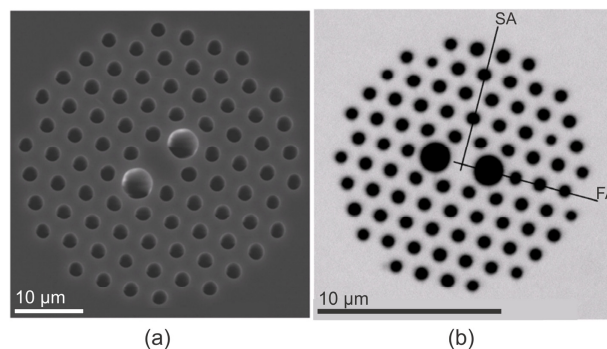
Fig. 1. Scanning electron micrographs of the commercially-available polarization maintaining PCF used in the experiments before (a) and after (b) tapering.
