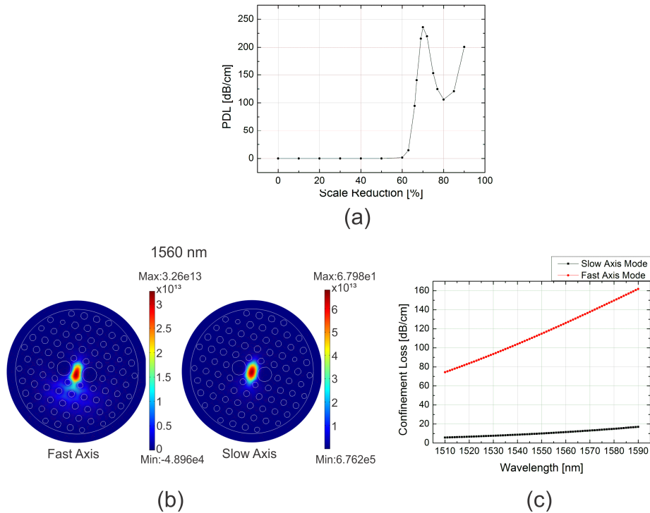
Fig. 2. (a) Simulated PDL as a function of the scale reduction factor. (b) Simulated light intensity distribution on the cross section of the tapered PCF. (c) Simulated confinement loss as a function of wavelength.
