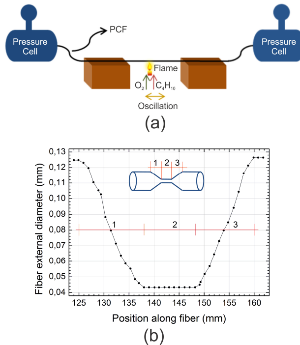
Fig. 3. (a) Tapering rig setup with differential pressure. (b) Tapered section profile: sections 1 and 3 are the transition regions, while section 2 is the down-tapered region with a constant diameter.
