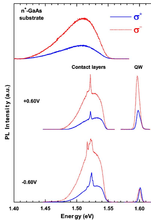
FIG. 2. (Color online) Typical \sigma^+ and \sigma^- PL spectra for an n^+ bulk GaAs substrate sample and from the RTD under a \pm 0.6 V bias voltage and 15 T.
