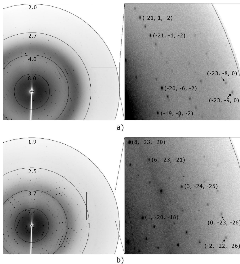
Figure 4. Typical diffraction images with resolutions circles drawn at 2.0 Å, 2.7 Å, 4.0 Å, 8.0 Å resolution for the P2_12_12_1 space group and 1.9 Å, 2.5 Å, 3.7 Å, 7.4 Å resolution for the P3_121 space group. a) A 1^\circ oscillation frame from P2_12_12_1 crystal form and b) a 0.4^\circ oscillation frame from P3_121 crystal form. A close-up of the outer edge including diffraction spots with their respective indices hkl is also shown.
