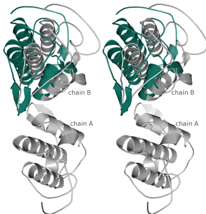
Figure 5. Stereo view of the superposition of the dimers present in the ASU of B j VIII crystals (space groups P3_121 and P2_12_12_1 ). The models shown were built from the search models after application of the molecular replacement solutions, as described in text. The transformation matrix calculated from the superposition of chain A in space group P2_12_12_1 onto the corresponding chain in space group P3_121 (fixed) was applied subsequently to the entire dimer present in the ASU of space group P2_12_12_1 . After transformation, chain A coordinates are coincident and, for clarity, for the space group P2_12_12_1 only the chain B is shown (colored in green). The entire dimer of the space group P3_121 is shown in gray. The figure unequivocally indicates a difference in the relative orientation of chain B with respect to the chain A. Figures were prepared using PyMOL (DeLano Scientific, San Carlos, CA, http://pymol.sourceforge.net ) and edited with GIMP ( http://www.gimp.org ) under Linux.
