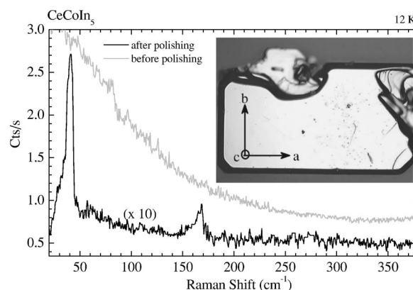
FIG. 1. Raman spectra of polished and unpolished monocrystals of \text{CeCoIn}_5 at 12 K. The spectral intensity of the polished crystal was multiplied by 10 for clarity. The inset shows a picture of a monocrystal of \text{CeCoIn}_5 . The a , b , and c crystallographic axes are also indicated.
