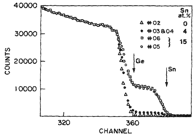
FIG. 1. Rutherford backscattering spectra from sputtered \alpha -Ge, \alpha -Ge:Sn, and \alpha -Ge:Sn:H homogeneous alloys (up to Sn/(Ge + Sn) ~ 0.15) deposited onto Corning 7059 glass and crystalline silicon substrates. The incident \alpha -particle beam energy and spectrometer resolution are 760 and 14 keV, respectively. The vertical arrows indicate the position in the RBS spectra of Sn and Ge at the surface.
