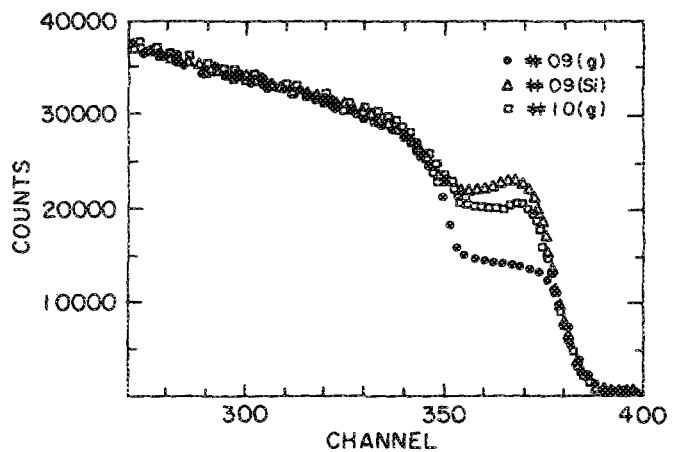
FIG. 2. Rutherford backscattering spectra of \alpha -Ge:Sn and \alpha -Ge:Sn:H showing a metal segregation at the outer surface. The spectrum of sample 09(g) (Sn/(Ge + Sn) ~ 0.27) showing no metallic segregation is also displayed. Measuring conditions are identical to those of Fig. 1.
