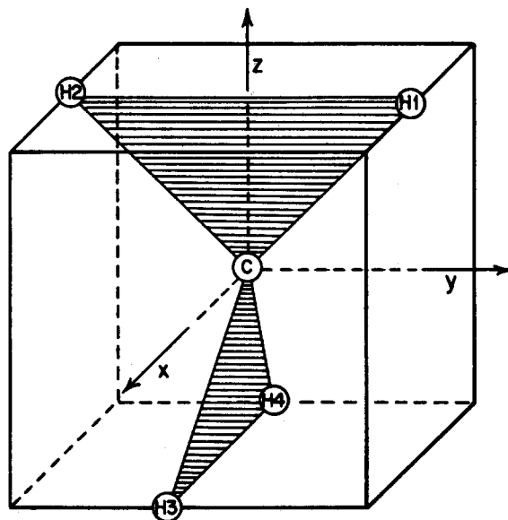
FIG. 2. Orientation of methane assumed in calculations.
