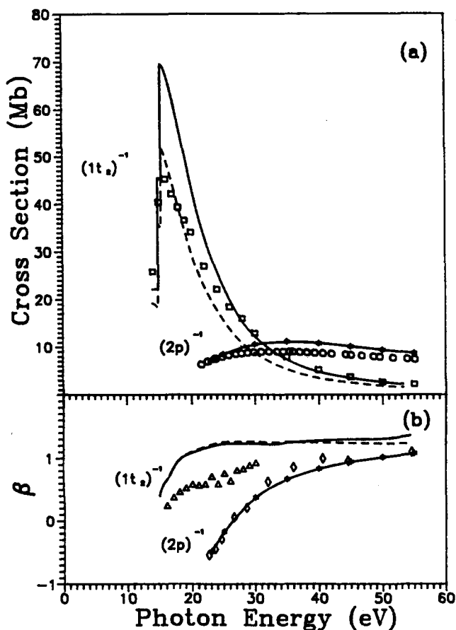
FIG. 1. (a) Cross sections for photoionization of the 1t_2 orbital of \text{CH}_4 and the 2p orbital of Ne: —, present results for \text{CH}_4 (dipole length); ---, present results for \text{CH}_4 (dipole velocity). See the Results and Discussion section for discussion of step-like behavior at threshold; \square , experimental data of Backx et al. (Ref. 3) for \text{CH}_4 ; \blacktriangle , present results for Ne (dipole length); \circ , experimental data of Marr et al. (Ref. 4) for neon. (b) Photoelectron asymmetry parameters for photoionization of the 1t_2 orbital of \text{CH}_4 and the 2p orbital of Ne: —, present results for \text{CH}_4 (dipole length); ---, present results for \text{CH}_4 (dipole velocity); \triangle , experimental data of Marr et al. (Ref. 10) for \text{CH}_4 ; \blacktriangle , present results for Ne; \diamond , experimental data of Codling et al. (Ref. 11) for Ne.
