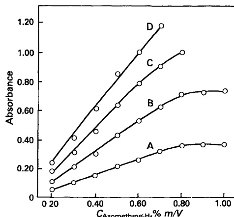
Fig. 4. Variation of the absorbance for various concentrations of azomethine-H in 2.0% ascorbic acid. Buffer-masking solution, 14.0% m/V (\text{NH}_4)_2\text{HPO}_4 in 5% EDTA; buffer pH = 8.1 \pm 0.2 ; residence time, 280 s; L_s = 300 \mu\text{l} . Boron concentrations: A, 1.00; B, 2.00; C, 3.00; and D, 4.00 \mu\text{g ml}^{-1} . The results are corrected against the blank values
