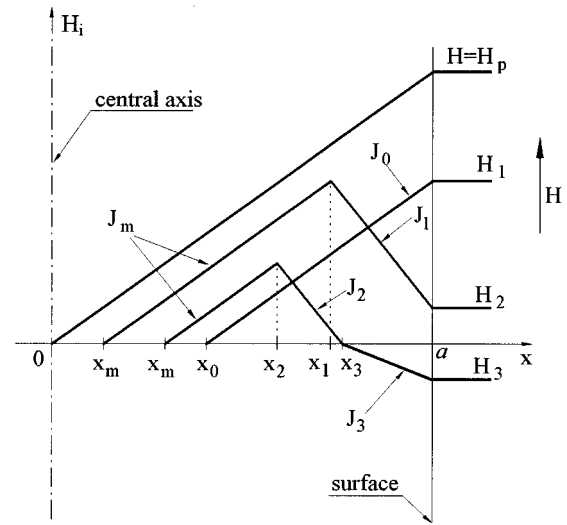
FIG. 1. Schematic view of typical profiles of the magnetic field inside the sample, as the external field varies from zero to H_1 , H_p , H_2 and H_3 . The supercurrent densities J_0 , J_m , J_1 , J_2 , and J_3 are associated with the field gradients in different regions (or layers) whose boundaries are located at points x = 0, x_0, x_1, x_2, x_3, a . The center and surface are located at x=0 and x=a , respectively.
