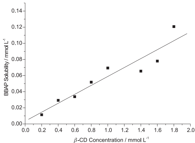
Figure 4. Solubility of BBAP in water at 25 °C as a function of \beta -CD concentration.
