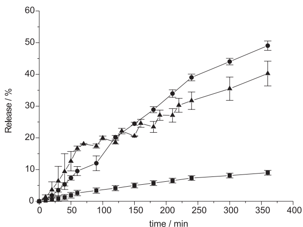
Figure 5. Dissolution profiles of BBAP (■), BBAP/ \beta -CD 1:1 (●) and 1:2 (▲), in water at 37 °C during six hours.
