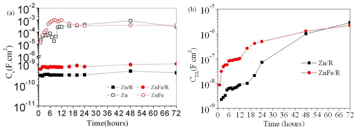
Figure 6: Time dependence of coating capacitance ( C_c ) and double-layer capacitance ( C_{DL} ) in a 3% NaCl solution. (a) C_c of resin coated and uncovered samples; (b) C_{DL} of Zn/R and ZnFe/R.
