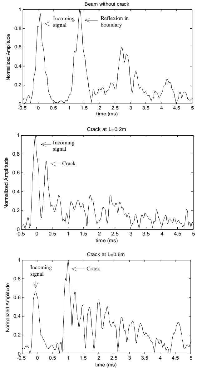
Figure 14. Envelope of level 2 DWT coefficients with mother wavelet db40 for beams without and with crack at positions L = 0.2 m and L = 0.6 m.
