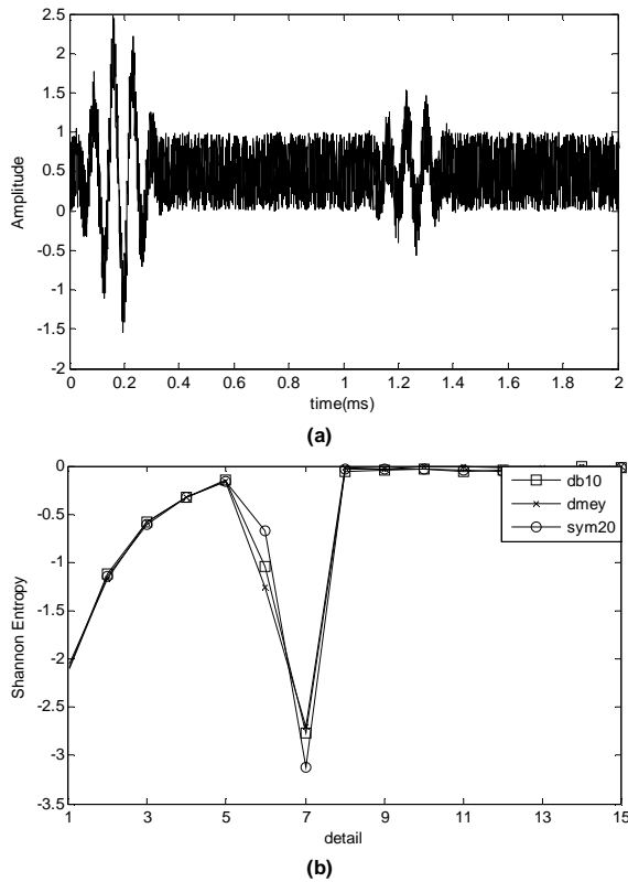
Figure 4. (a) Analyzed Signal; (b) Shannon entropy of DWT coefficients for mother wavelets Db10, discrete Meyer and Symlet 20.
