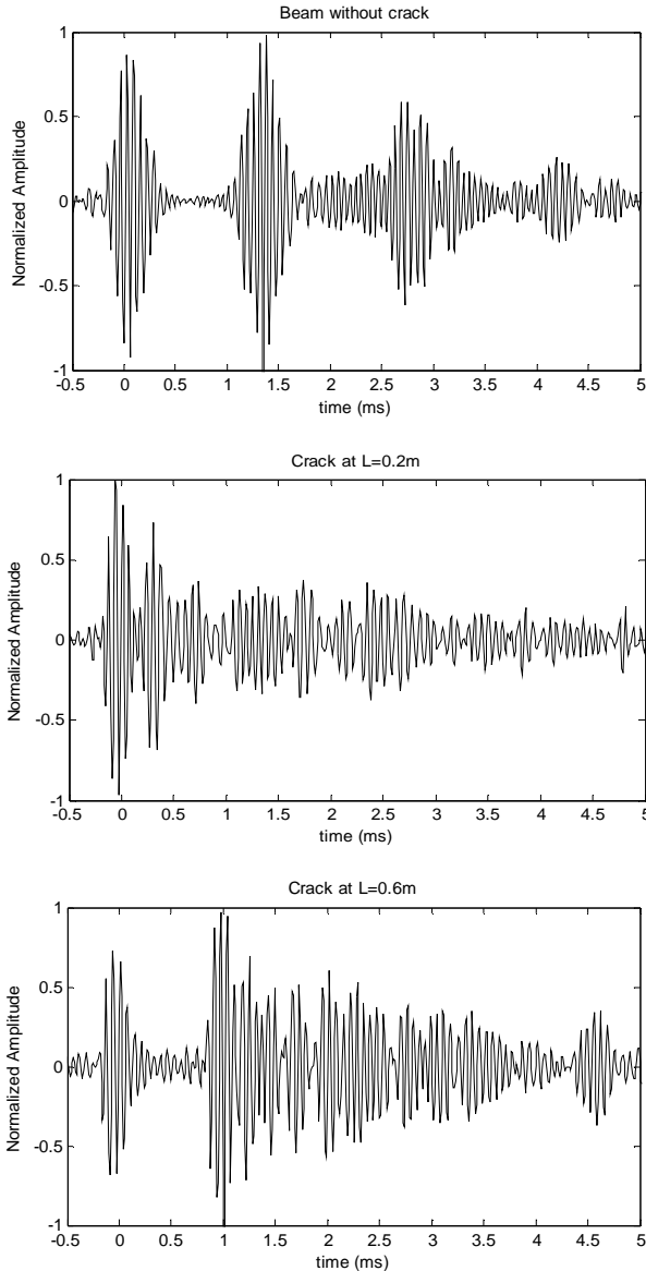
Figure 13. DWT coefficients of level 2 using the mother wavelet db40 for beams without and with crack at positions L = 0.2 m and L = 0.6 m.
