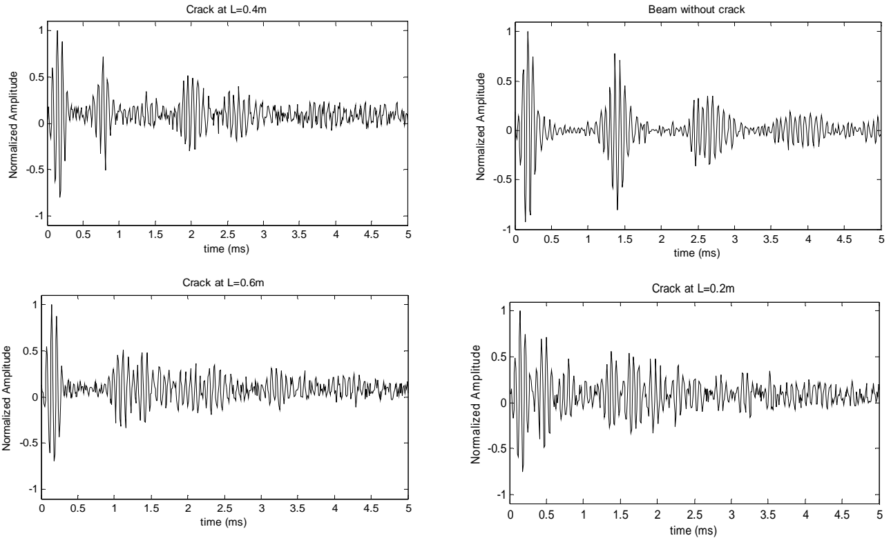
Figure 6. Wave propagation signal obtained by SFEM modeling for beams without and with crack at positions L = 0.2 m, L = 0.4 m and L = 0.6 m.
