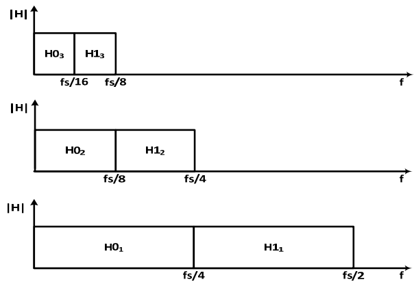
Figure 3. Frequency range of High and Low pass filters for 3 levels of decomposition.
