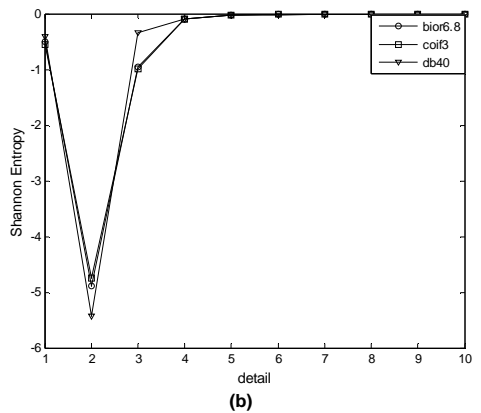
Figure 12. Shannon's entropy of the DWT coefficients for beam (a) without crack; (b) with crack at 0.6 m.
