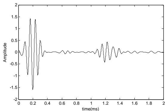
Figure 5. Detail level 7 coefficients of DWT with mother wavelet Symlet 20.
