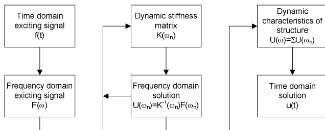
Figure 1. SFEM flow diagram for wave propagation in structures.
