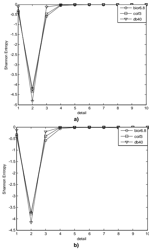
Figure 7. Shannon entropy of the DWT coefficients for beam (a) without crack; (b) with crack at 0.6 m.
