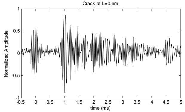
Figure 11. Experimental measurements of beams without and with crack at positions 0.2 m and 0.6 m.
