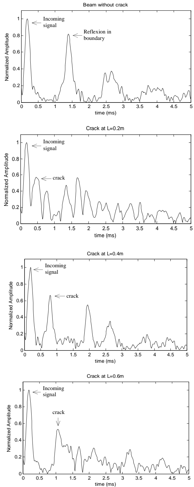
Figure 9. Envelope of level 2 DWT coefficients with mother wavelet db40 for beams without and with crack at positions L = 0.2 m, L = 0.4 m and L = 0.6 m.
