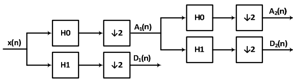
Figure 2. Two level analysis filter bank for DWT.
