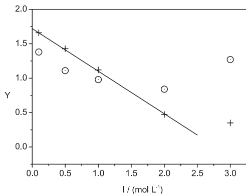
Figure 2. Plots of (O) Y = \log \beta and (+) Y = \log \beta - \Phi_{\text{Cu}} - \Phi_{\text{F}} as functions of the ionic strength I , for the \text{CoNCS}^+ system.
