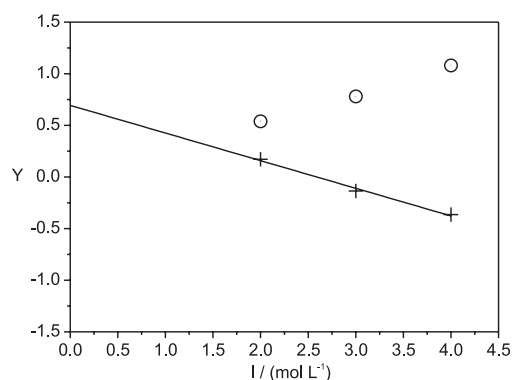
Figure 3. Plots of (O) Y = \log \beta and (+) Y = \log \beta - \Phi_{\text{Cu}} - \Phi_{\text{F}} as functions of the ionic strength I , for the \text{PbNCS}^+ system.
