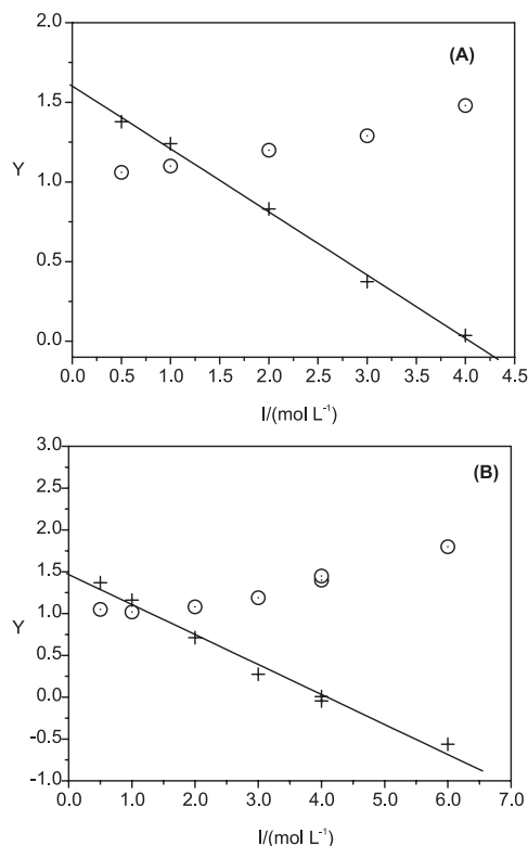
Figure 1. Plots of (o) Y = \log \beta and (+) Y = \log \beta - \Phi_{Cu} - \Phi_F as functions of the ionic strength I, for (A) the PbBr^+ system and (B) the SnCl^+ system.
