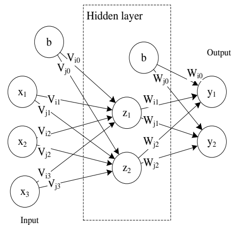
Figure 2. Backpropagation architecture.
