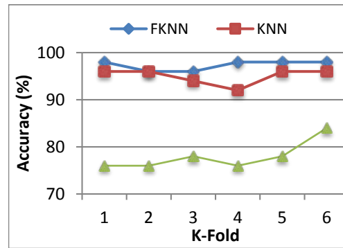
Figure 12. Comparison accuracy of FKNN, KNN and SVM.
