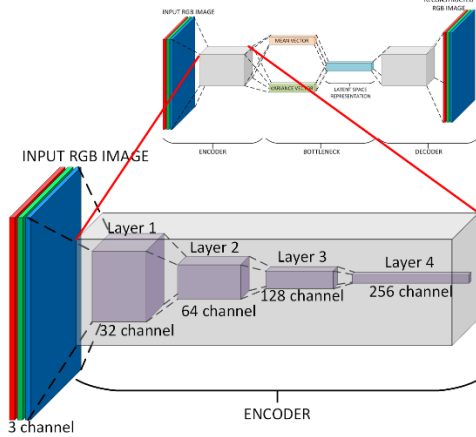
Figure 4. The structure inside encoder of the proposed Fully Convolutional Autoencoder for feature extraction of fire image datasets.
