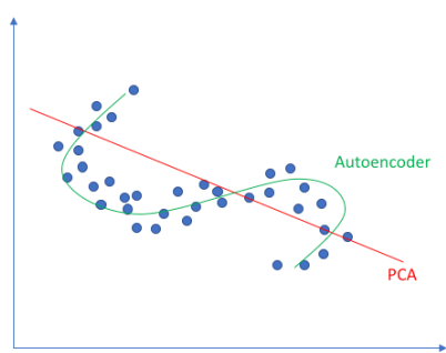
Figure 1. Comparison between PCA and Autoencoder [15]
