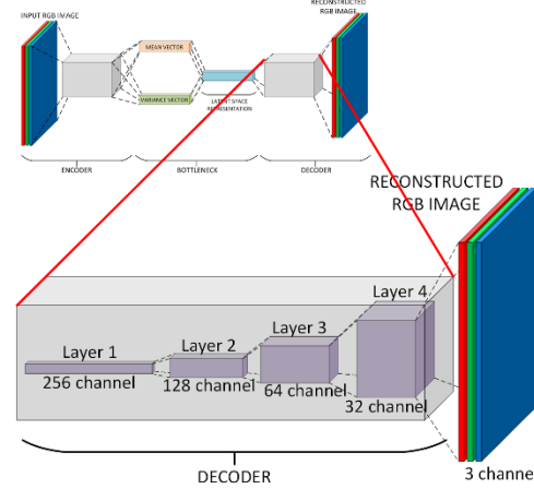
Figure 5. The structure inside decoder of the proposed Fully Convolutional Autoencoder for feature extraction of fire image datasets.
