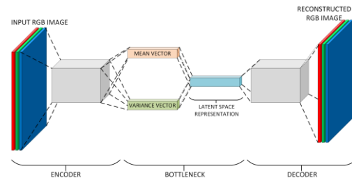
Figure 3. The structure of the proposed Fully Convolutional Autoencoder for feature extraction of fire image datasets.
