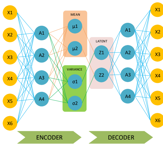
Figure 2. Basic structure of Variational Autoencoder (VAE)
